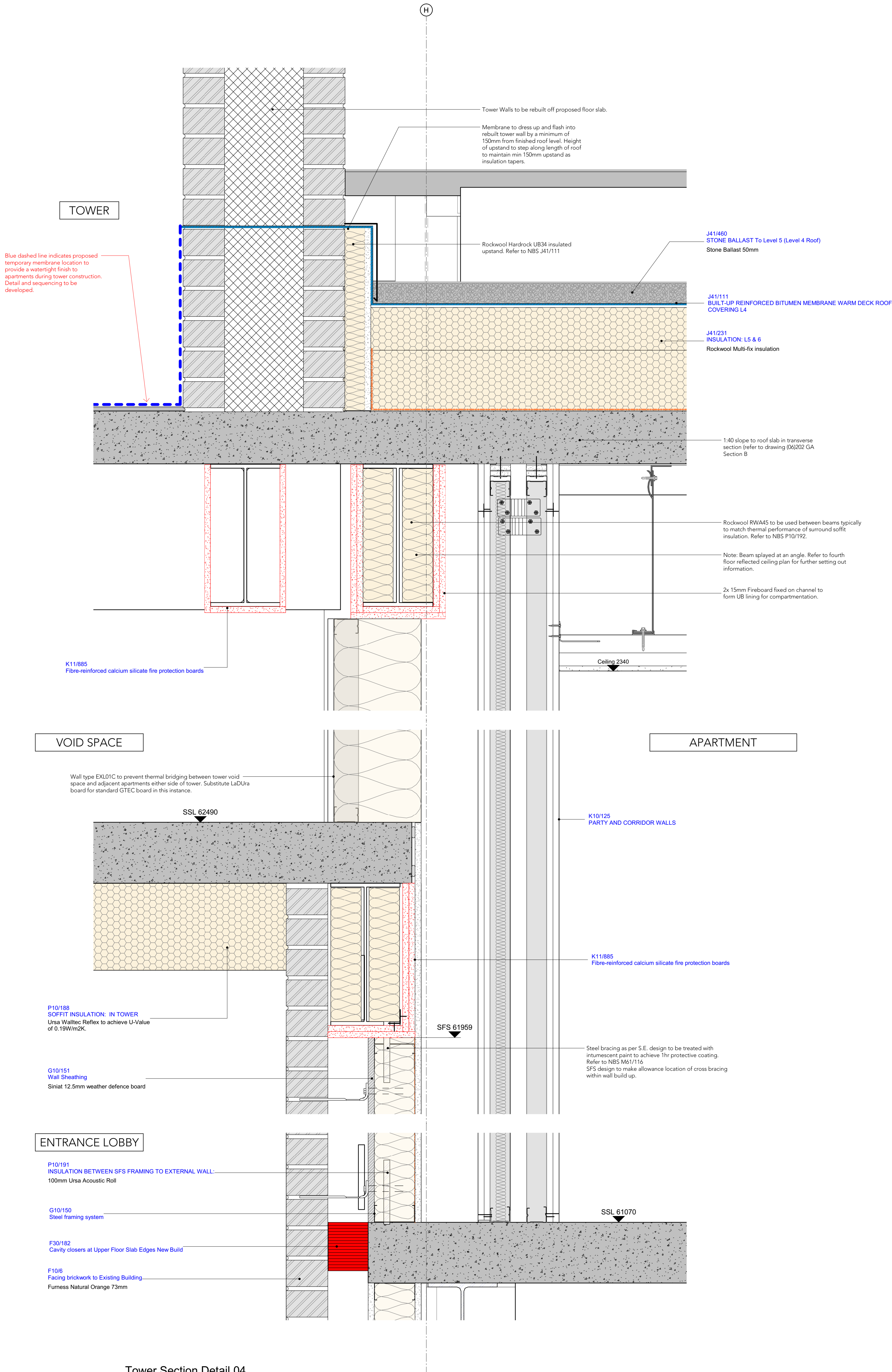
Tower Section Detail 04 1 : 5
