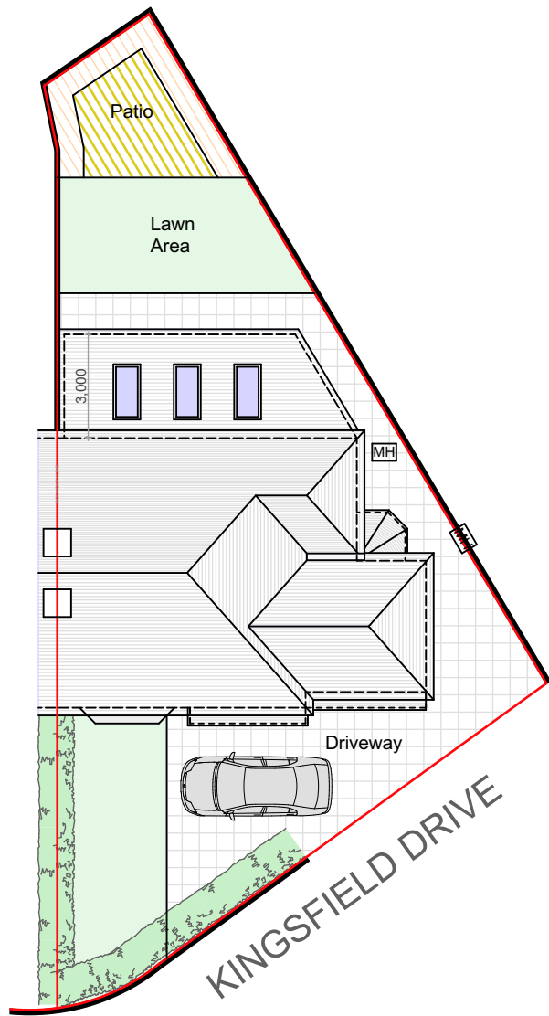
PROPOSED GA SITE PLAN @1:200
