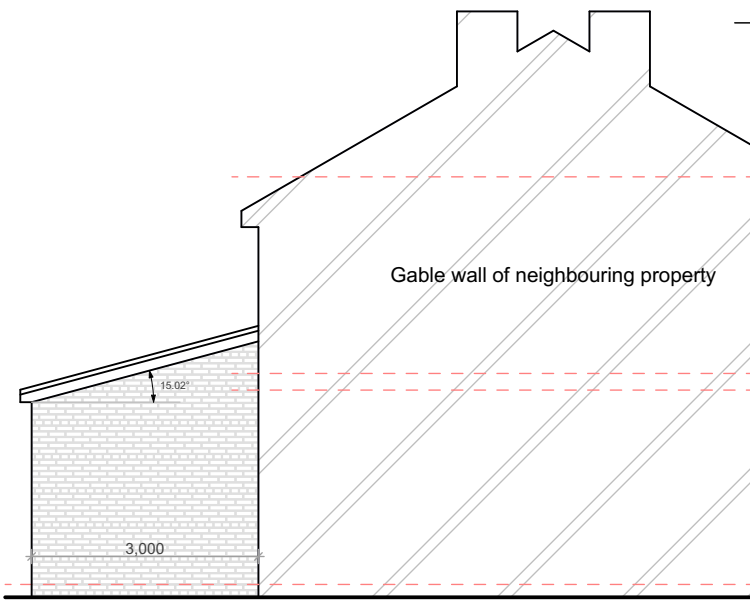
PROPOSED GA SIDE ELEVATION 2 @1:100
