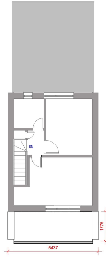
2 First Floor 1 : 100
