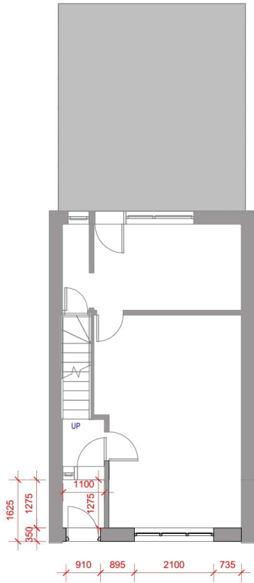
1 Ground Floor 1 : 100
