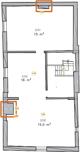
NORTH WING - SECOND FLOOR PLAN AS EXISTING
