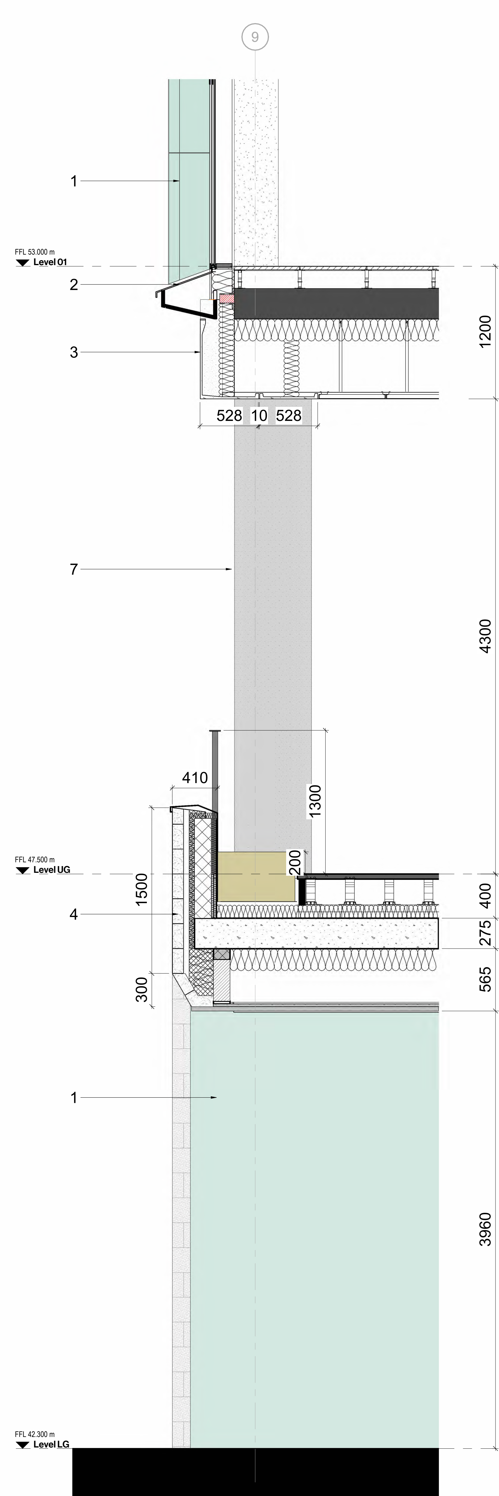
2 Lower Ground Bay Section.
