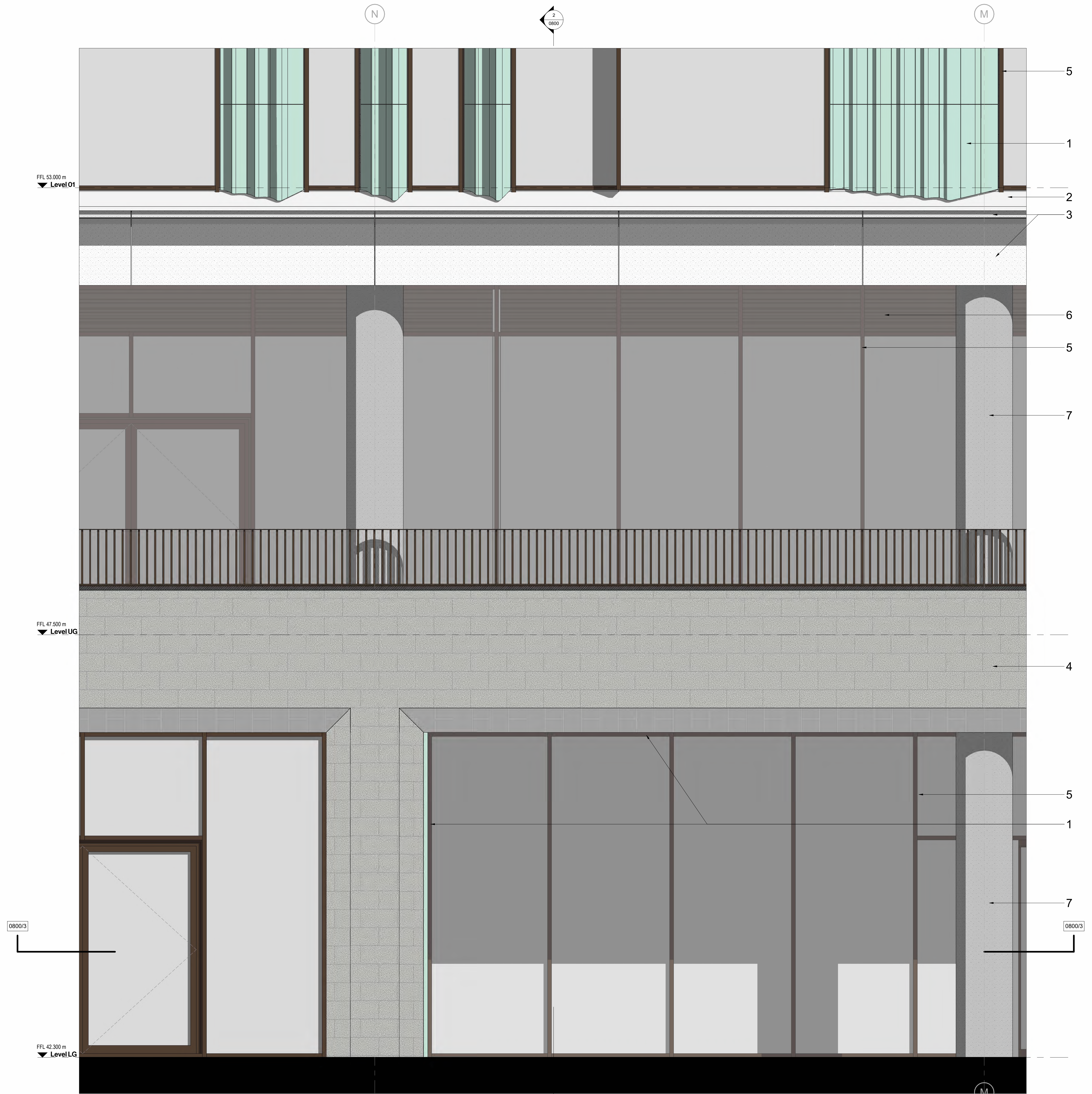
1 Lower Ground Bay Study
