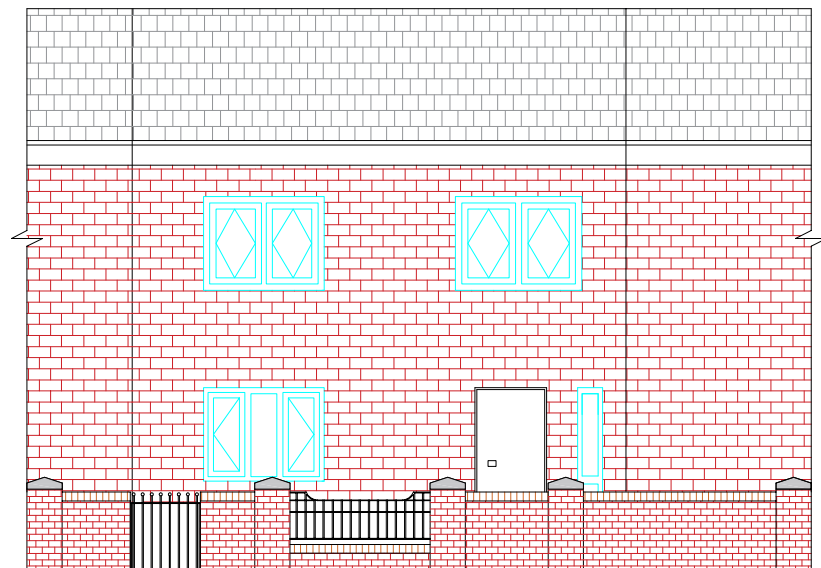
West Elevation
