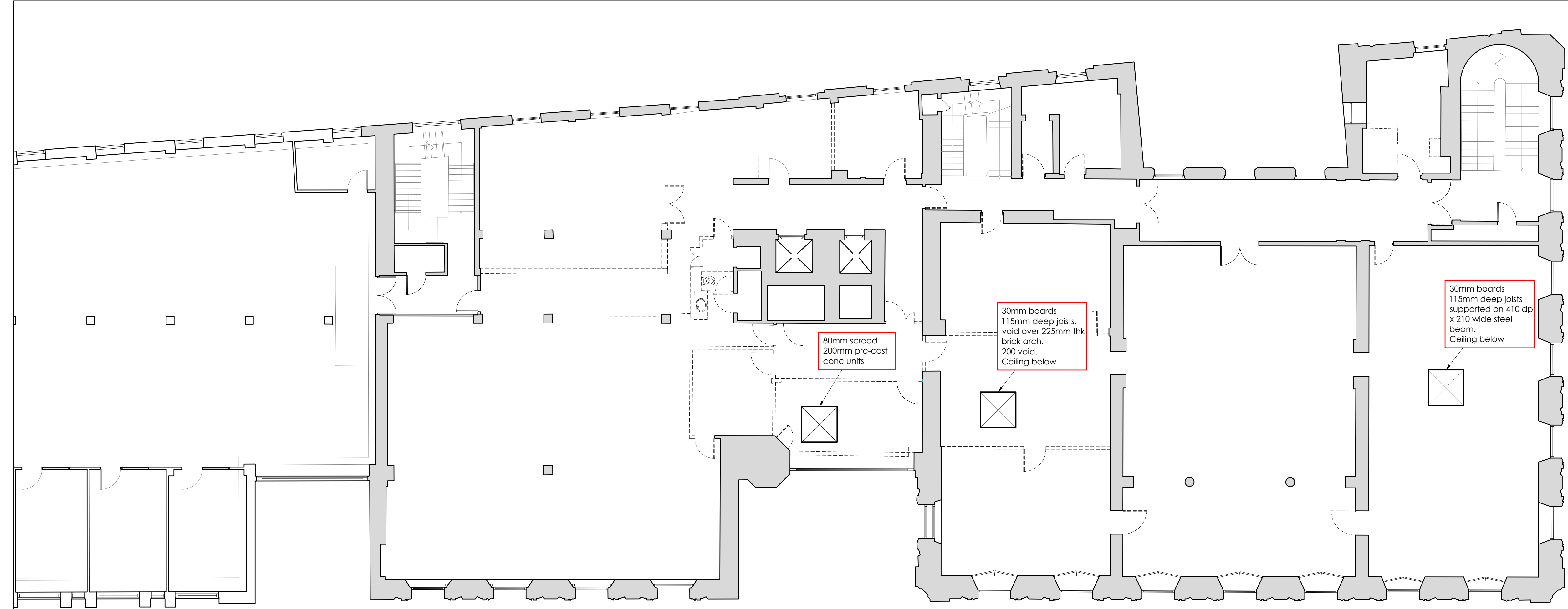
Second Floor - Existing Original Floor Construction 1:100 at A1
