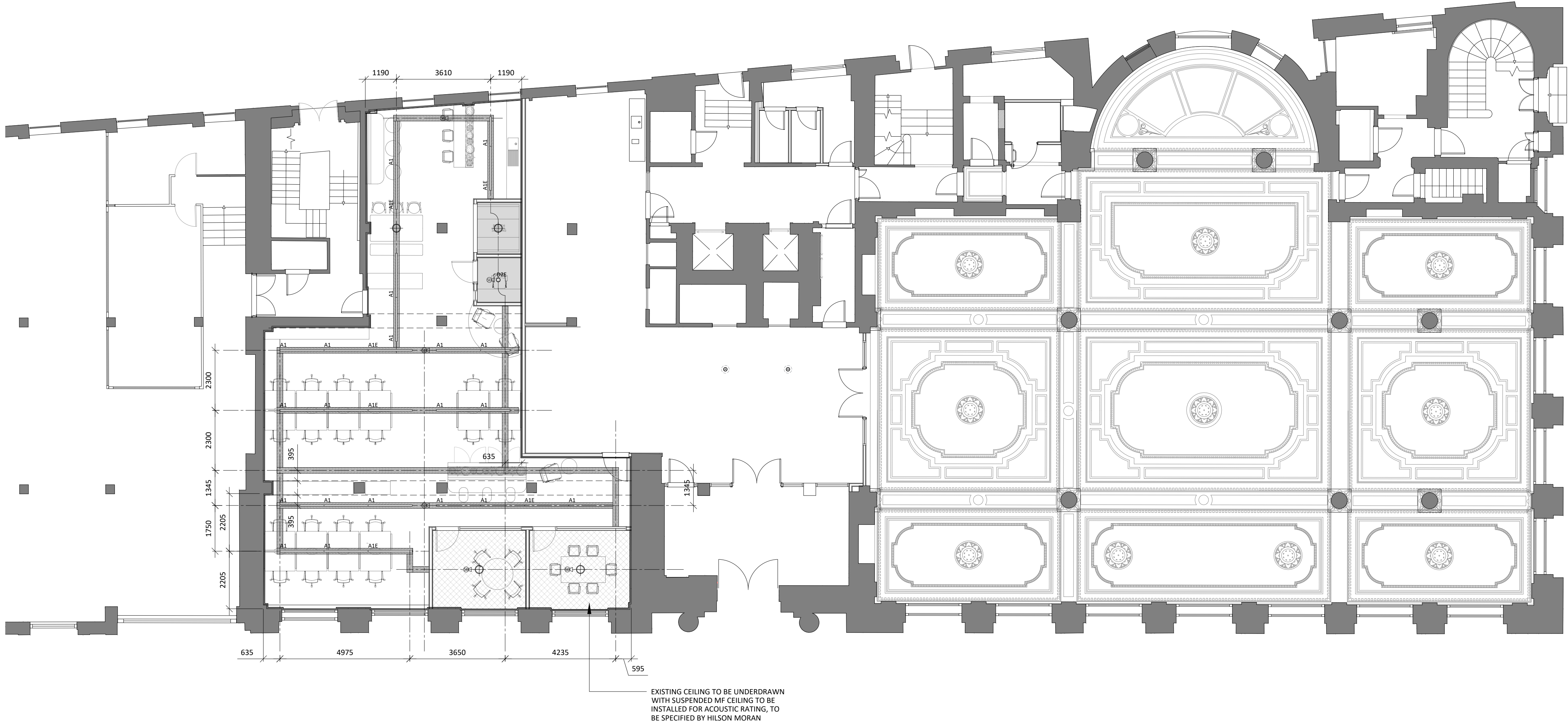
01 GROUND FLOOR RCP AS PROPOSED B300 SCALE - 1:100 @ A1 PLAN
