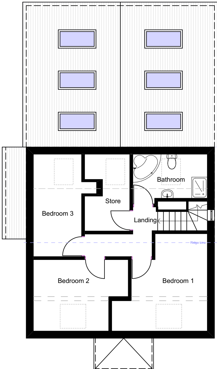
PROPOSED GA FIRST FLOOR PLAN
