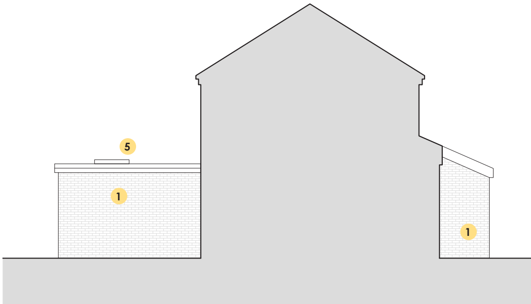
PROPOSED SIDE ELEVATION FROM 17 ATHERSTONE AVE 1:100 @ A3
