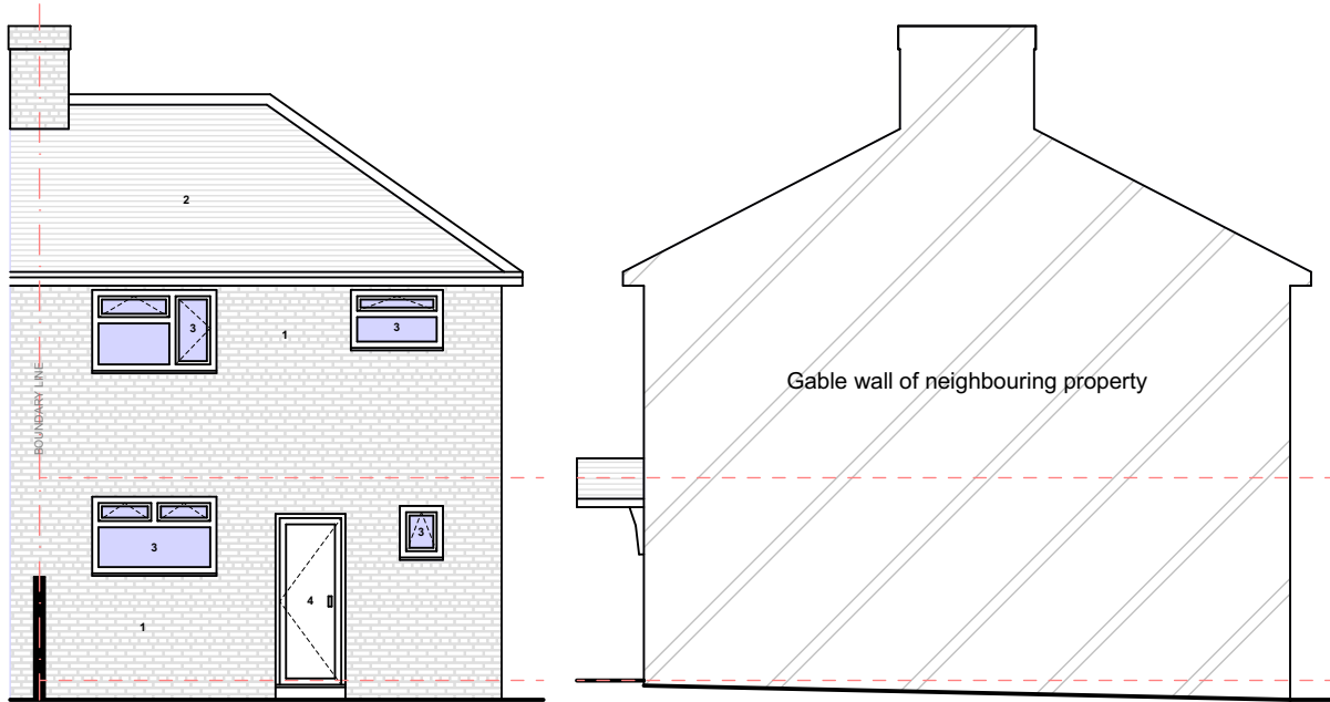
EXISTING GA REAR ELEVATION @1:100
