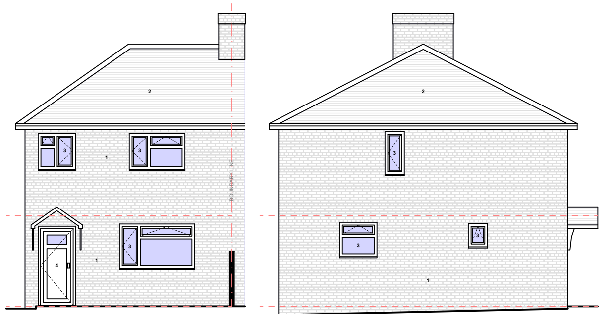
EXISTING GA FRONT ELEVATION @1:100
