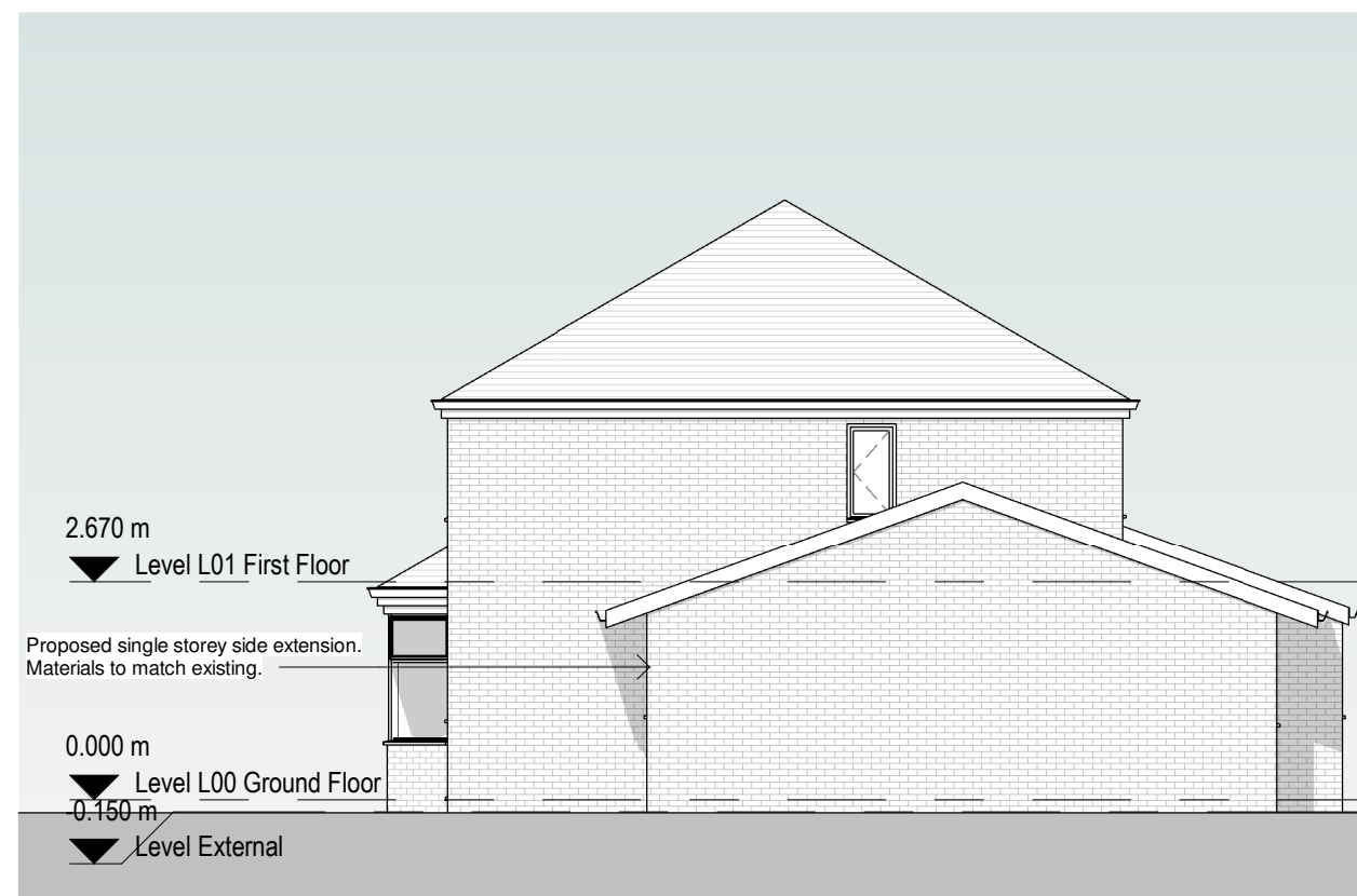
4 Proposed South Elevation 1 : 100
