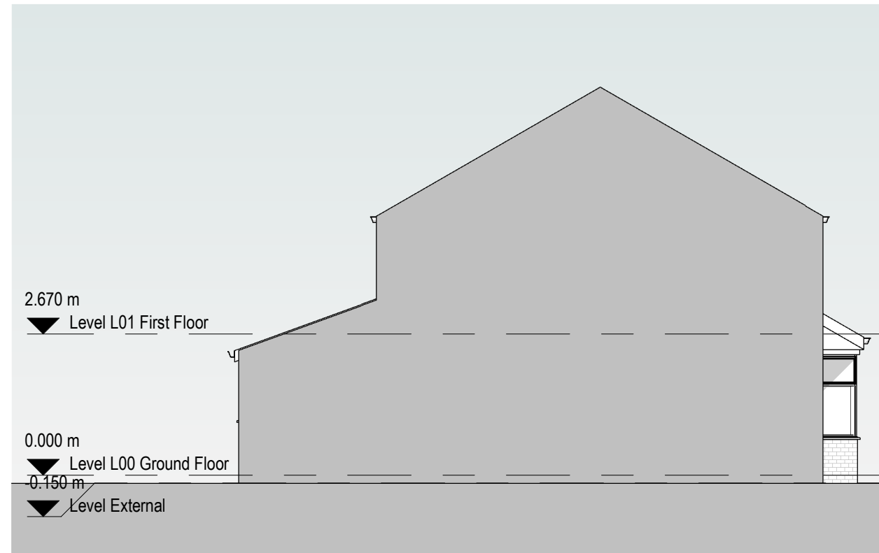
2 Proposed North Elevation 1 : 100
