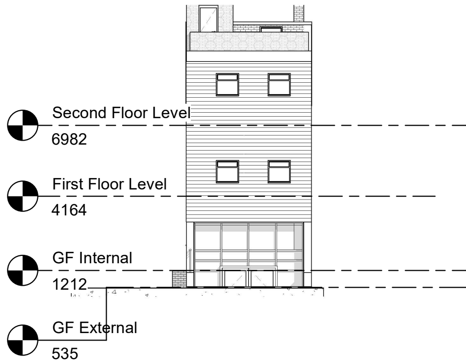
3 Rear Existing 1 : 150
