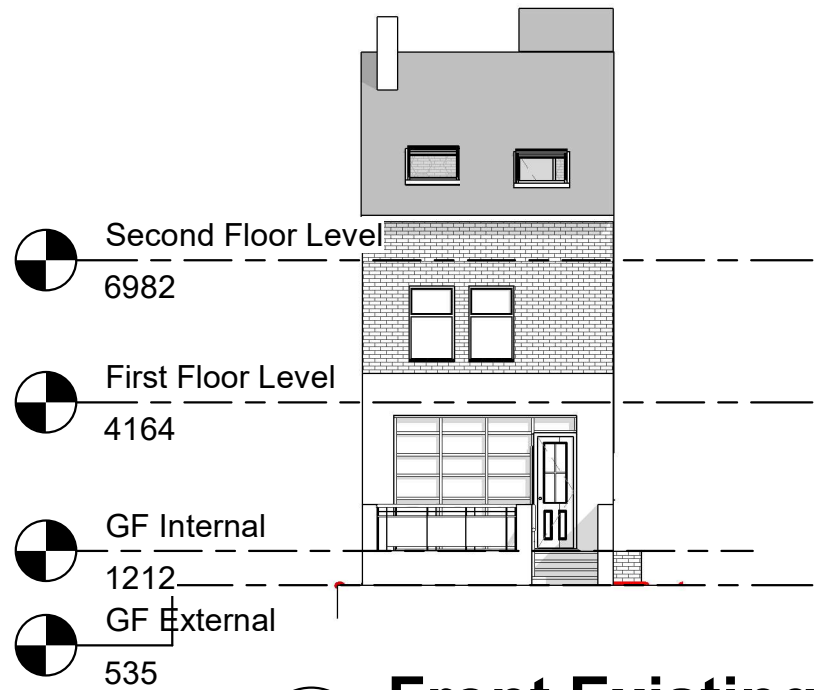
1 Front Existing 1 : 150
