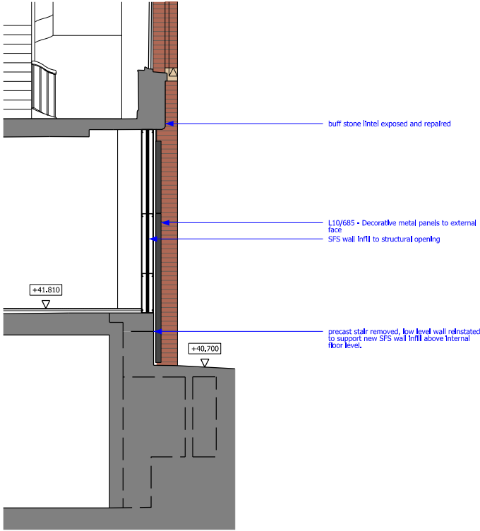
Proposed Section A-A 1:50
