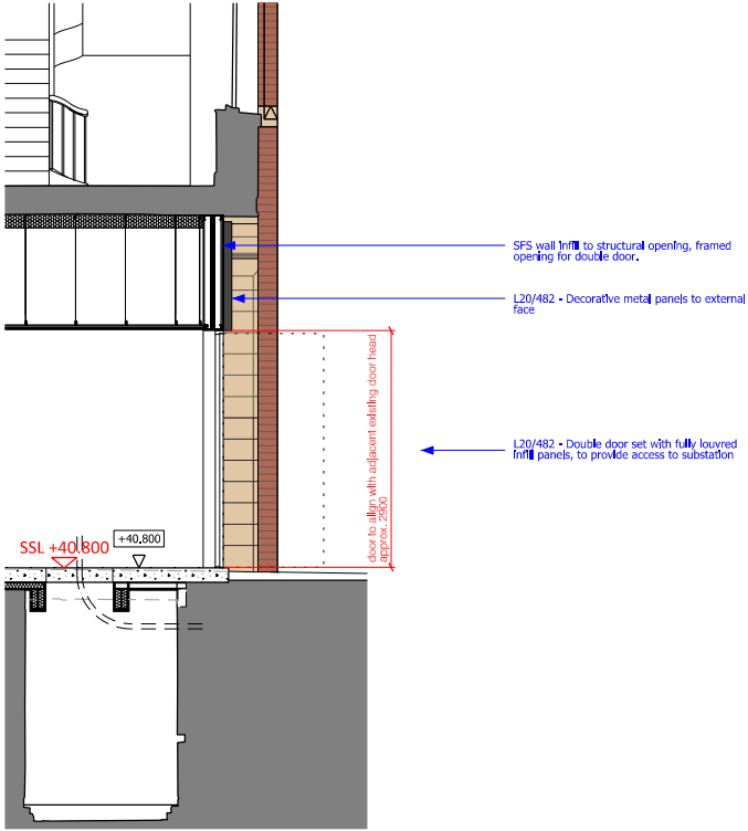
Proposed Section B-B 1:50
