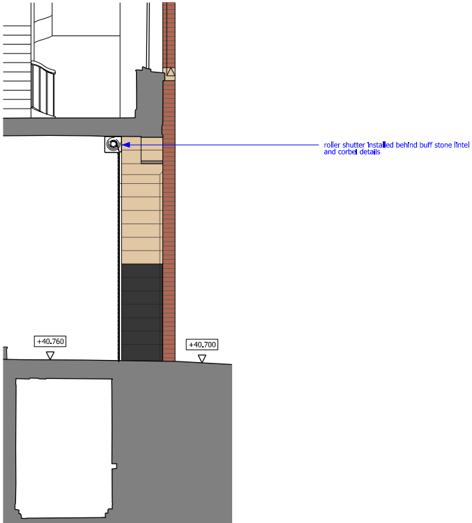
Existing Section B-B 1:50
