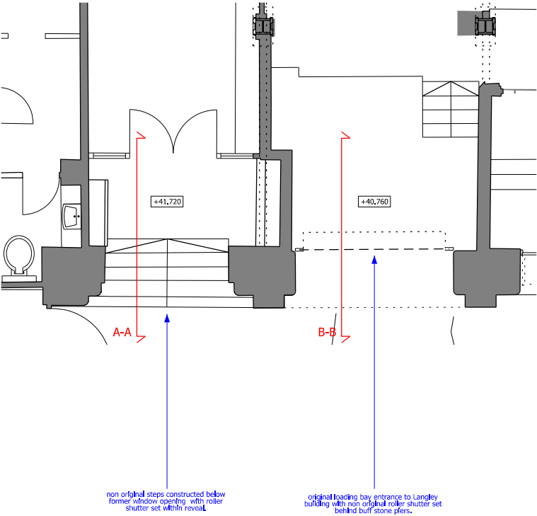
Existing Plan - Level -01 1:50
