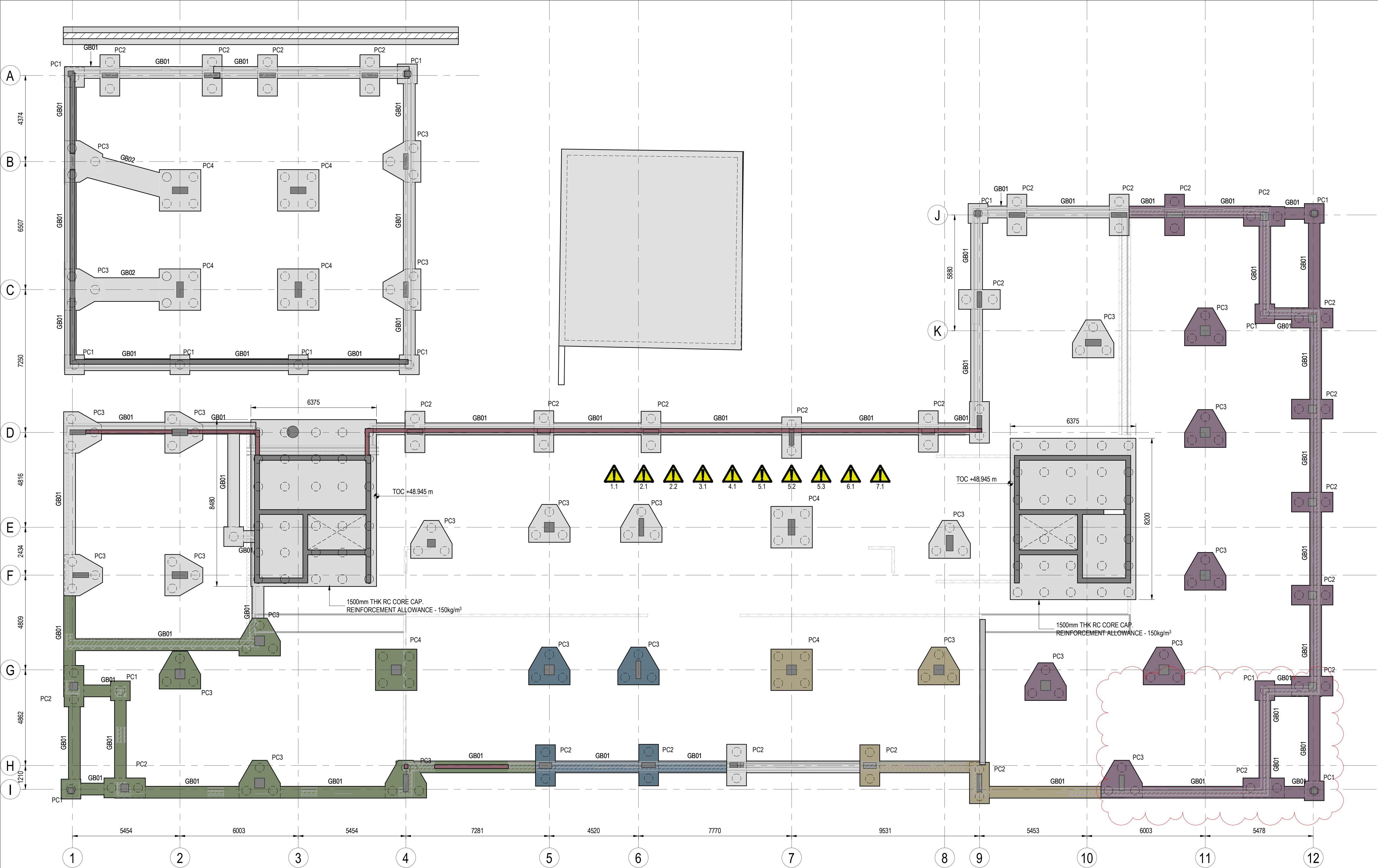
FOUNDATION GENERAL ARRANGEMENT SCALE: 1 : 100
