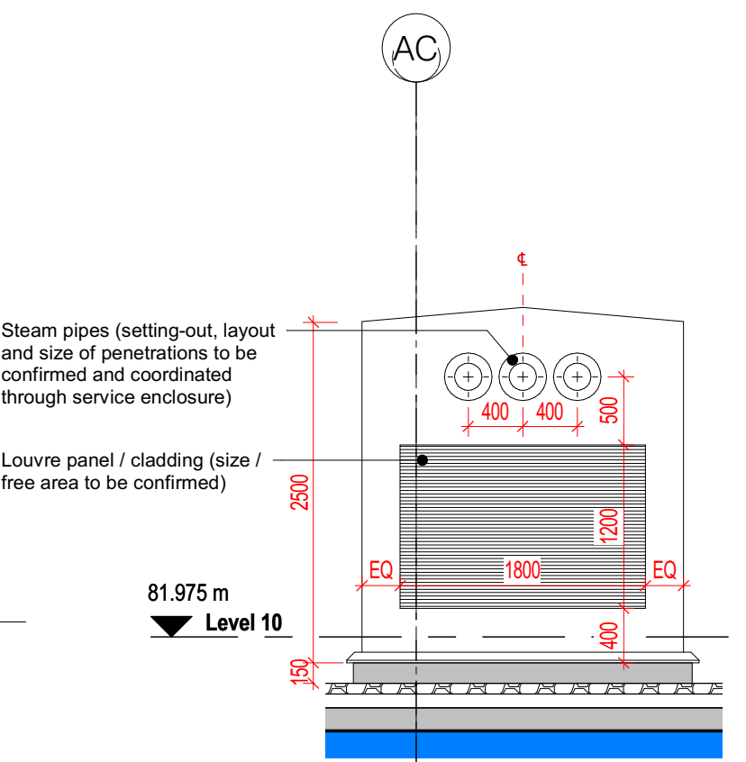
SE2 - Elevation 1
