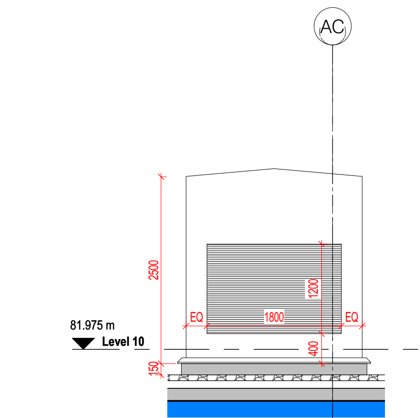
SE2 - Elevation 3
