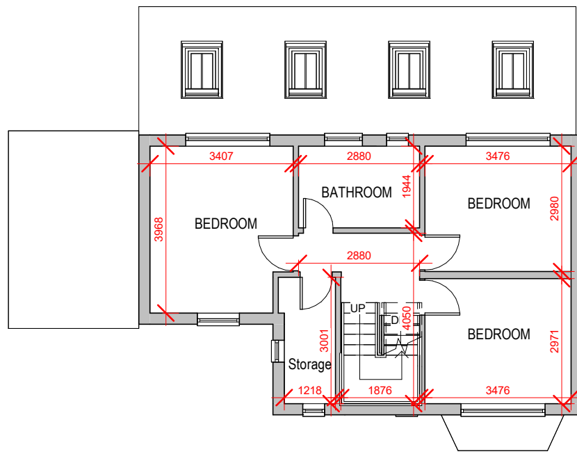
2 First Floor Plan 1 : 125
