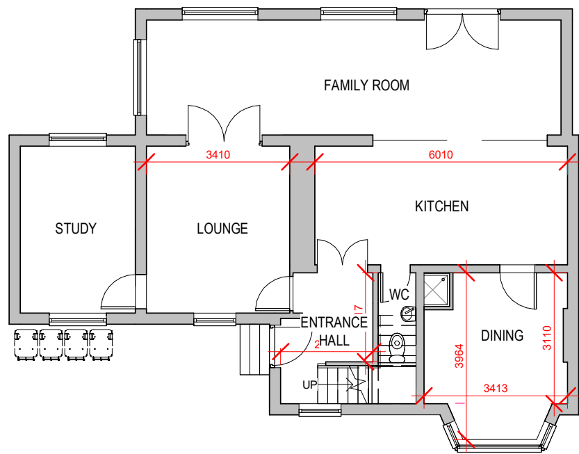
1 Ground Floor Plan 1 : 125
