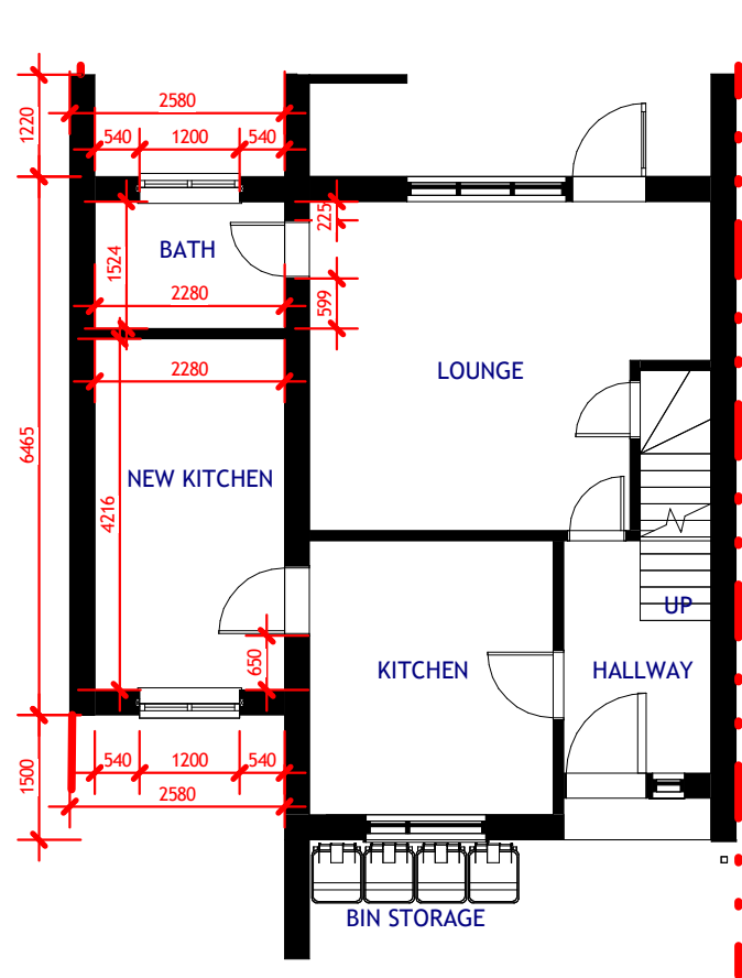
1 Ground Floor proposed 1 : 100
