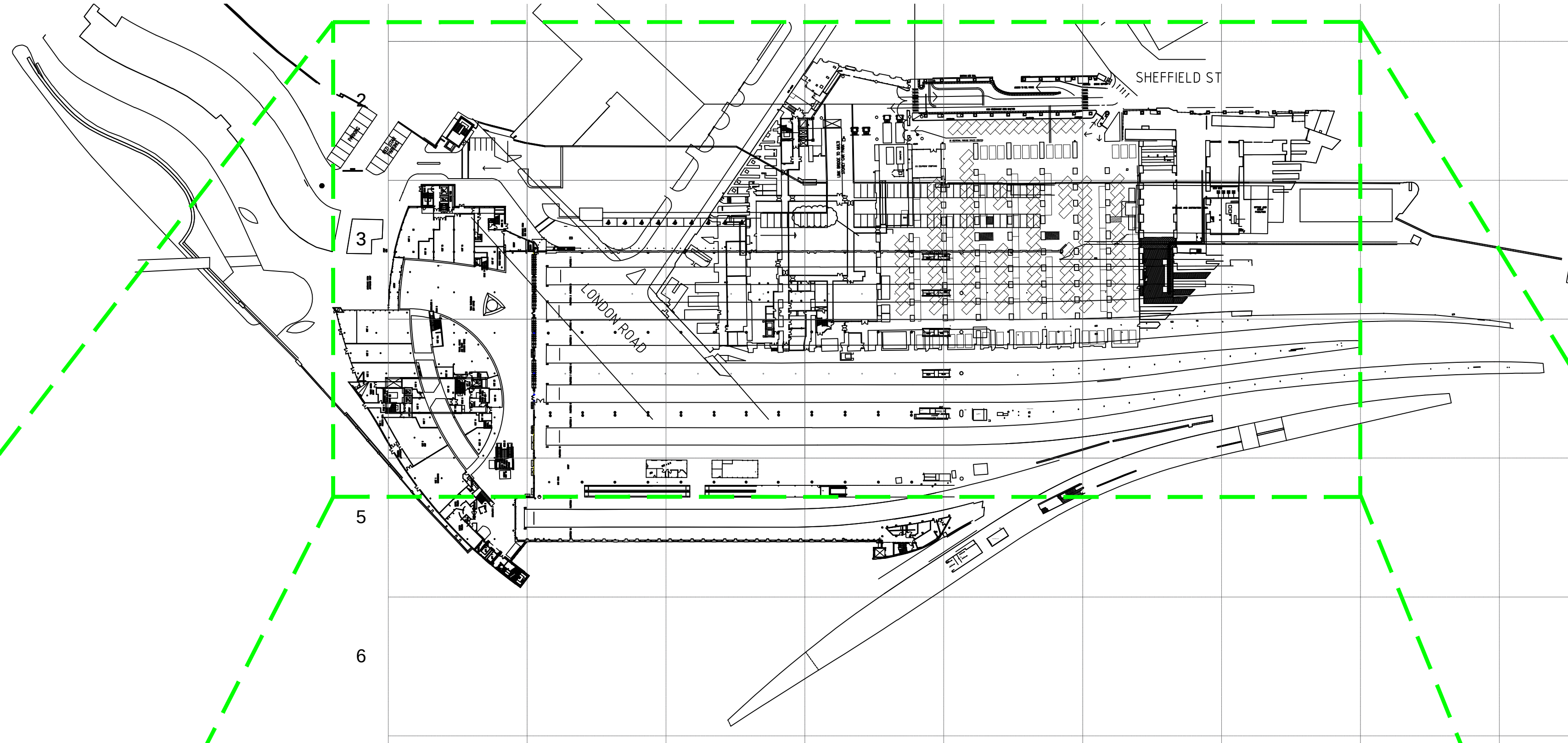
MANCHESTER PICCADILLY STATION LOCATION PLAN SCALE 1:1250
