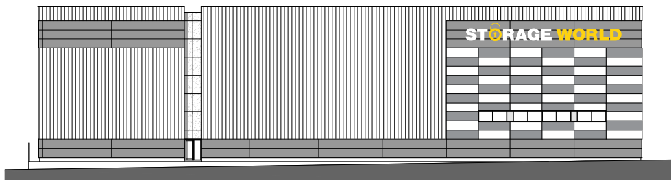
04 Proposed North Elevation
