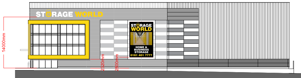
03 Proposed South Elevation
