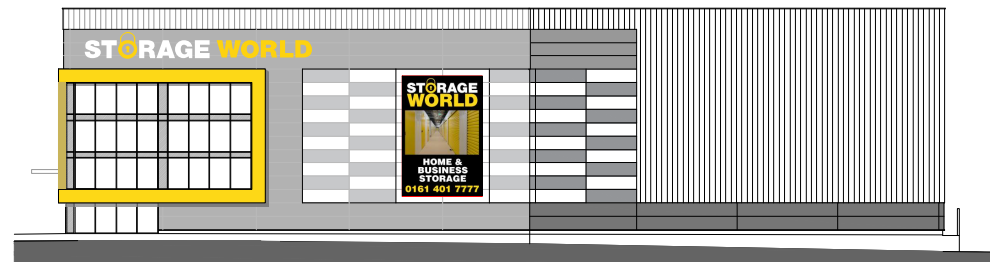
03 Proposed South Elevation
