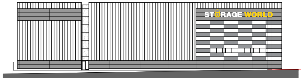
04 Proposed North Elevation
