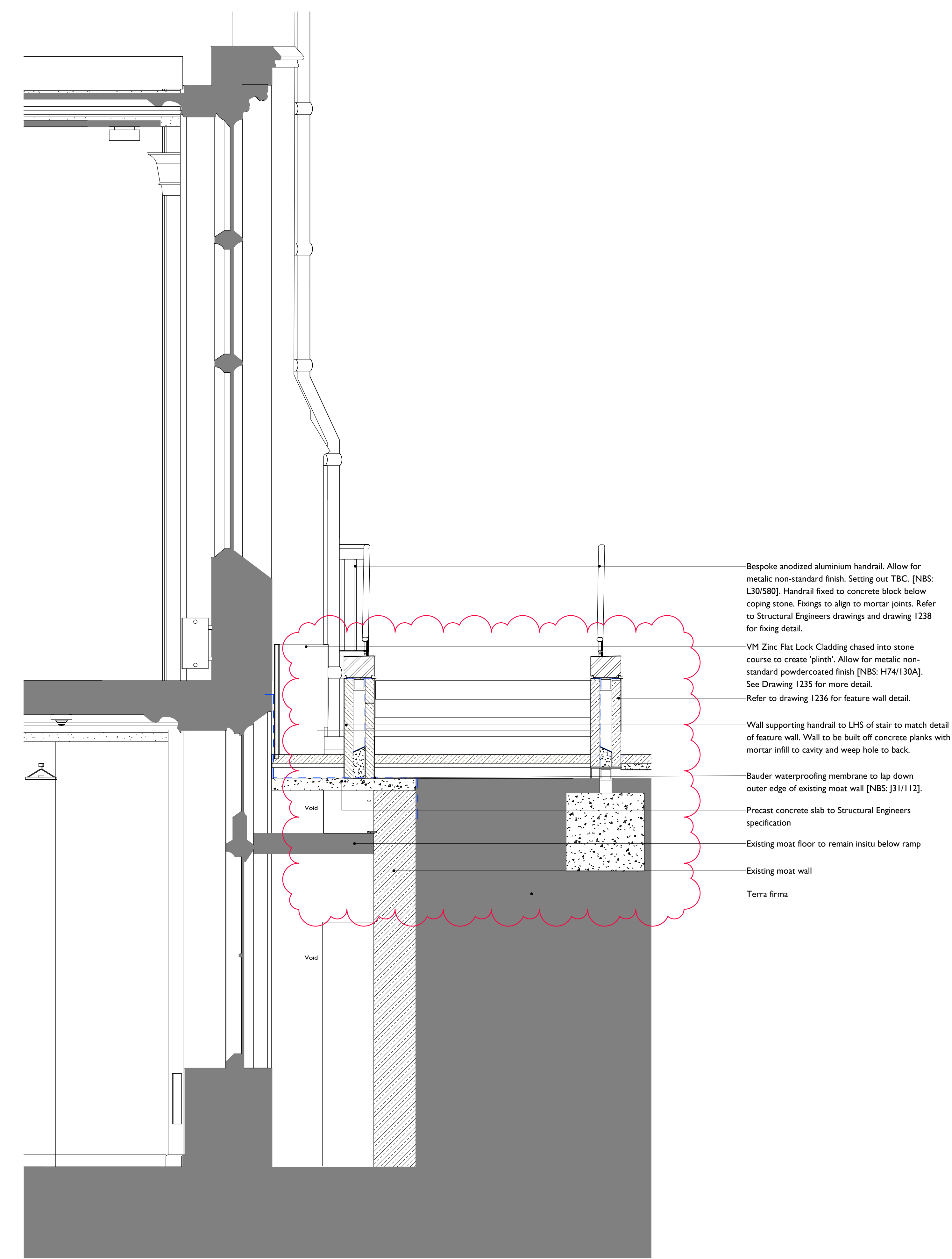
1 1237 Section HH as Proposed 1 : 20
