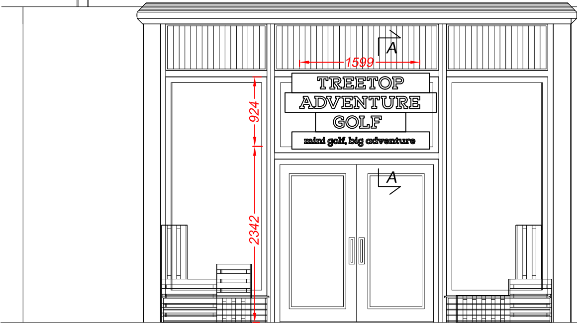
Dantzie St Elevation Scale 1:50
