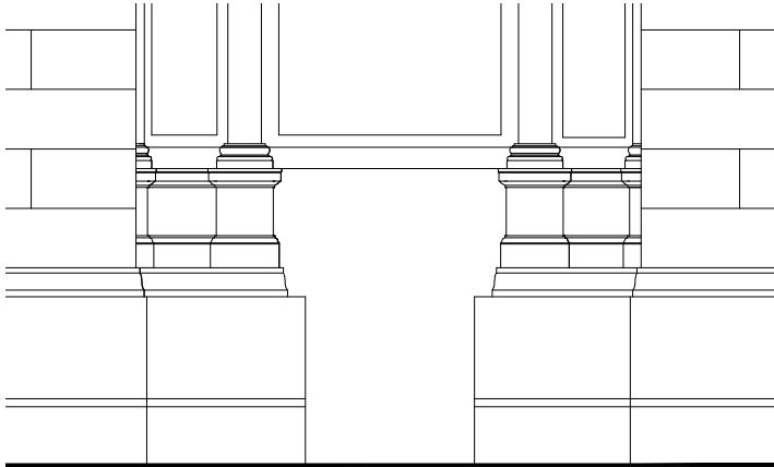
2 PROPOSED FRONT ELEVATION EXTRACT 1:25 @ A1 1:50 @ A3
