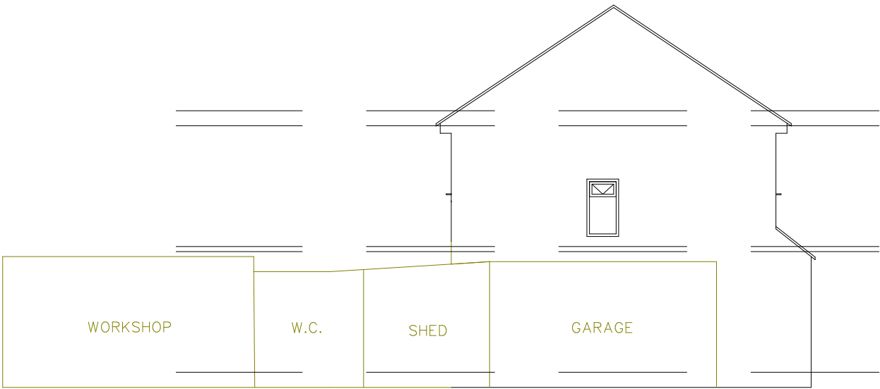
SIDE ELEVATION ELEVATION (from No.6)(A3 1:100)
