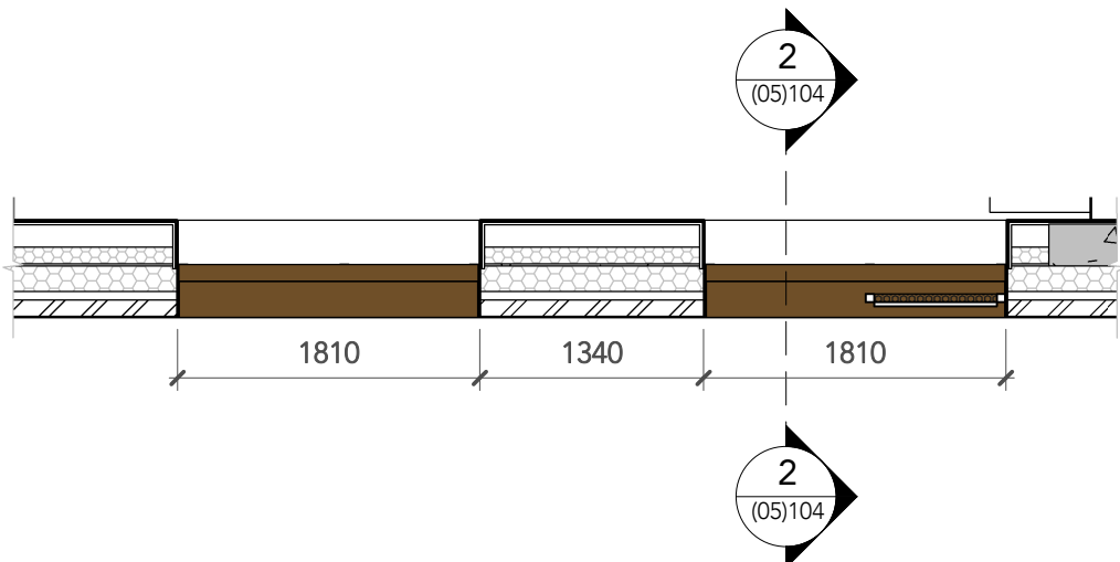
3 Bay Study Plan 1 : 50
