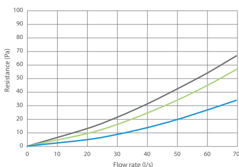
IAQBOX-D (1 outlet spigot)
