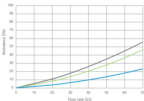
IAQBOX-D (2 outlet spigot)
