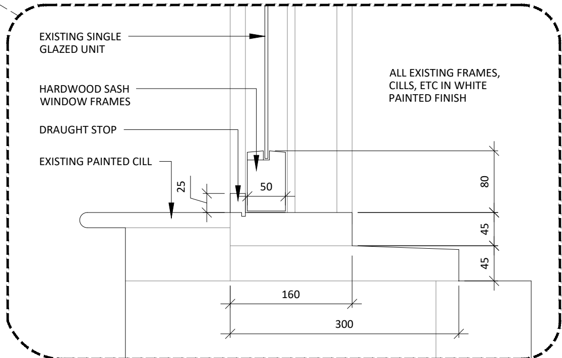
03c TYPE B WINDOW CILL 511 SCALE 1:5 EXISTING SECTION
