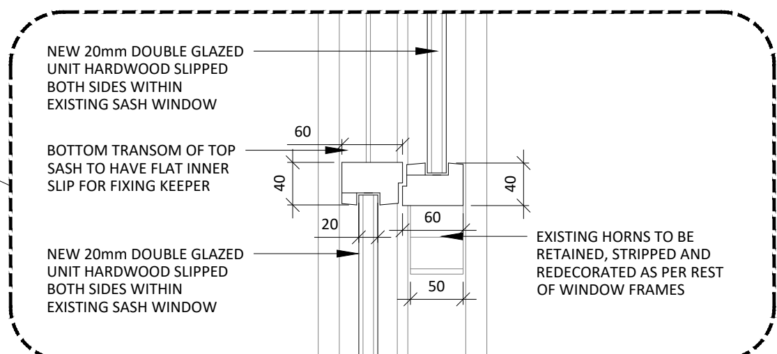
07b TYPE B WINDOW JOINT 511 SCALE 1:5 PROPOSED SECTION
