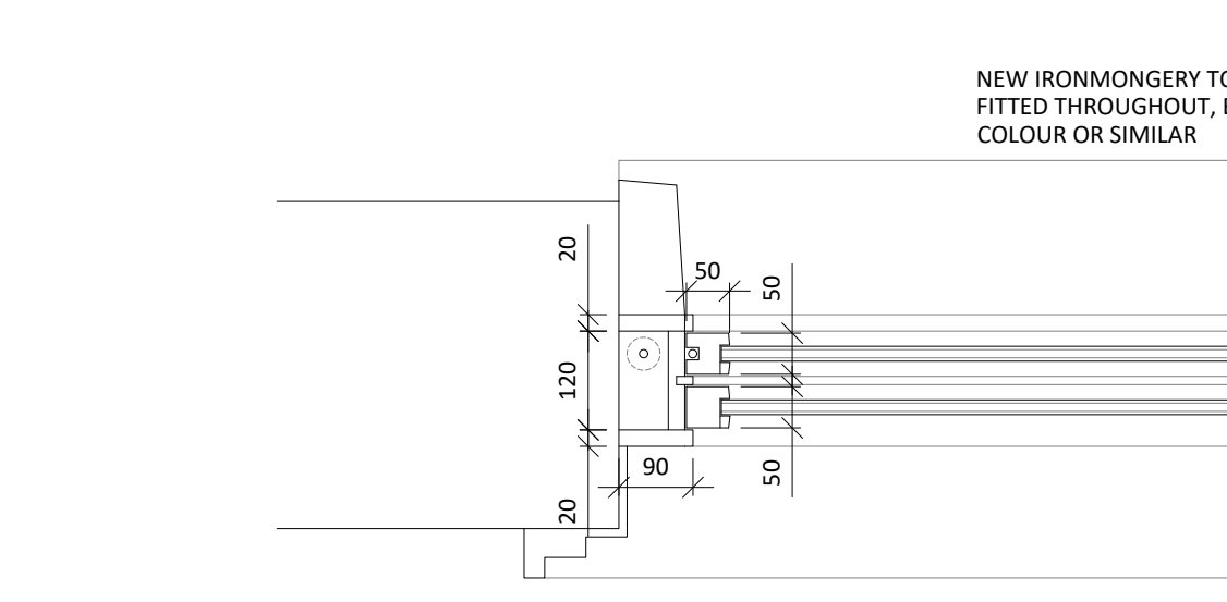
05 2nd FLOOR SASH WINDOW - TYPE B 511 SCALE 1:20 PROPOSED ELEVATION
