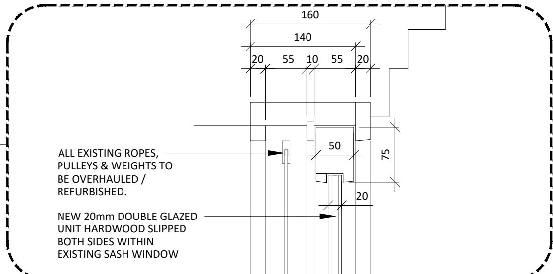
07a TYPE B WINDOW HEAD 511 SCALE 1:5 PROPOSED SECTION
