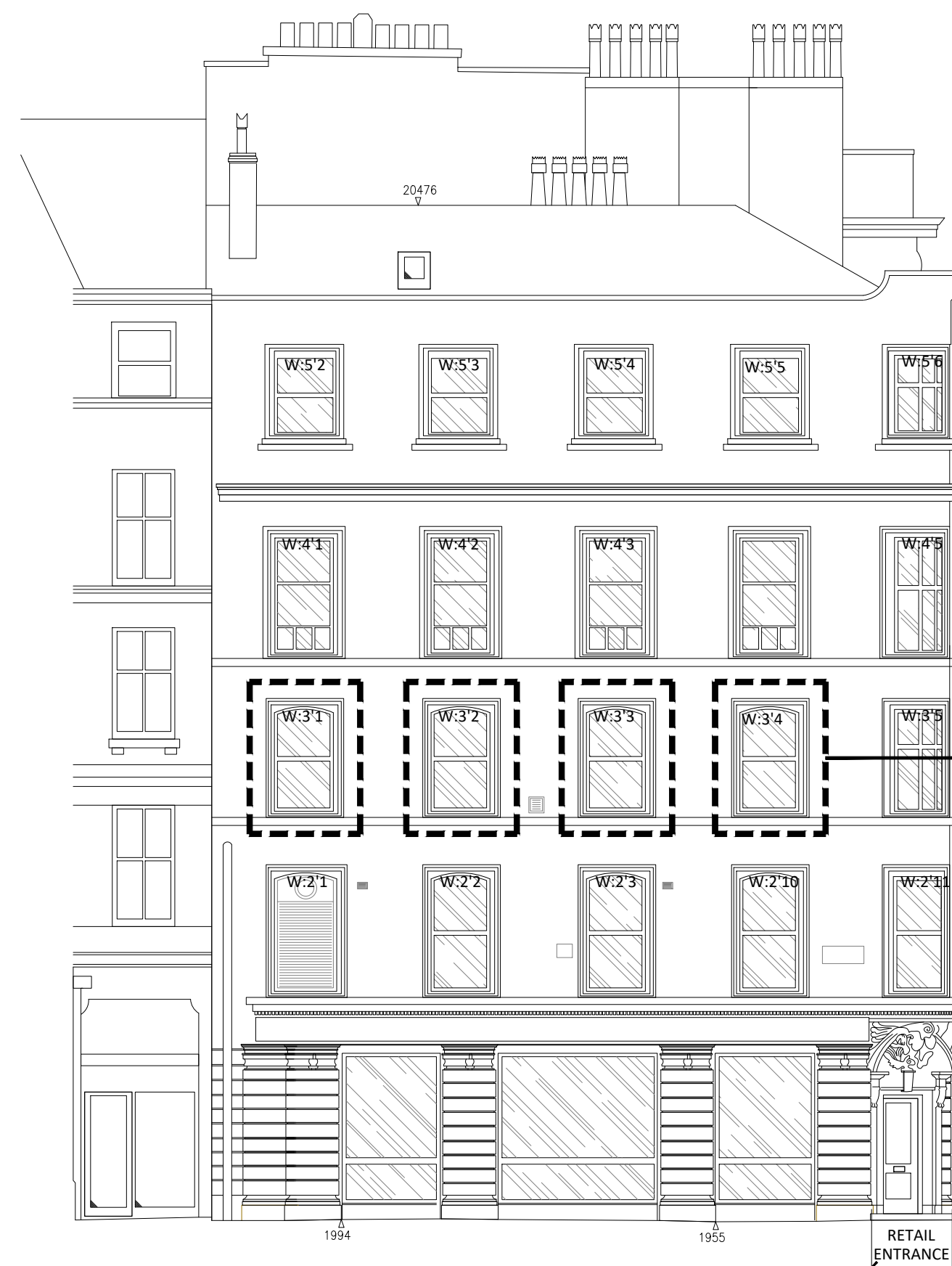
10 ST MARY'S STREET ELEVATION 511 SCALE 1:100
