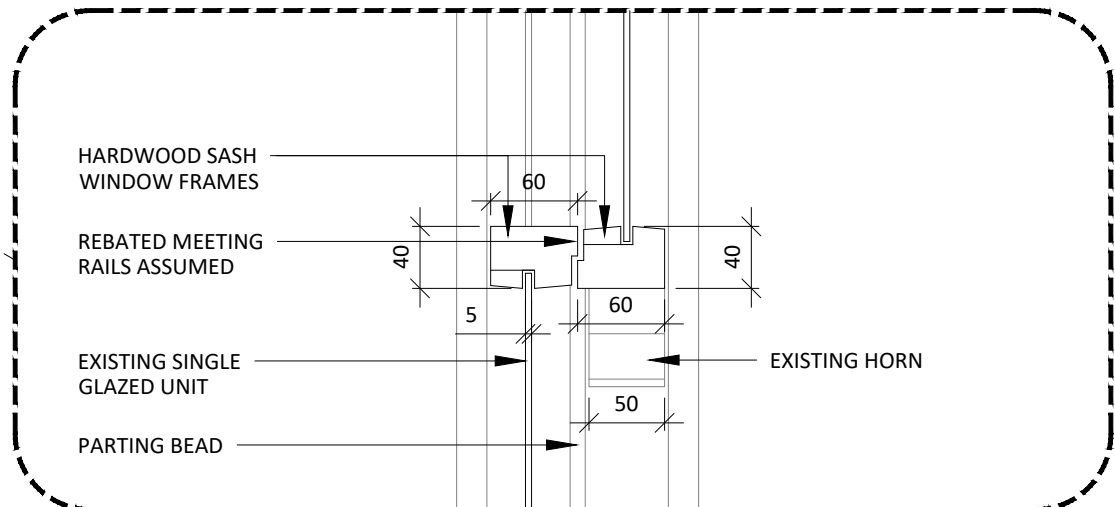
03b TYPE B WINDOW JOINT 511 SCALE 1:5 EXISTING SECTION
