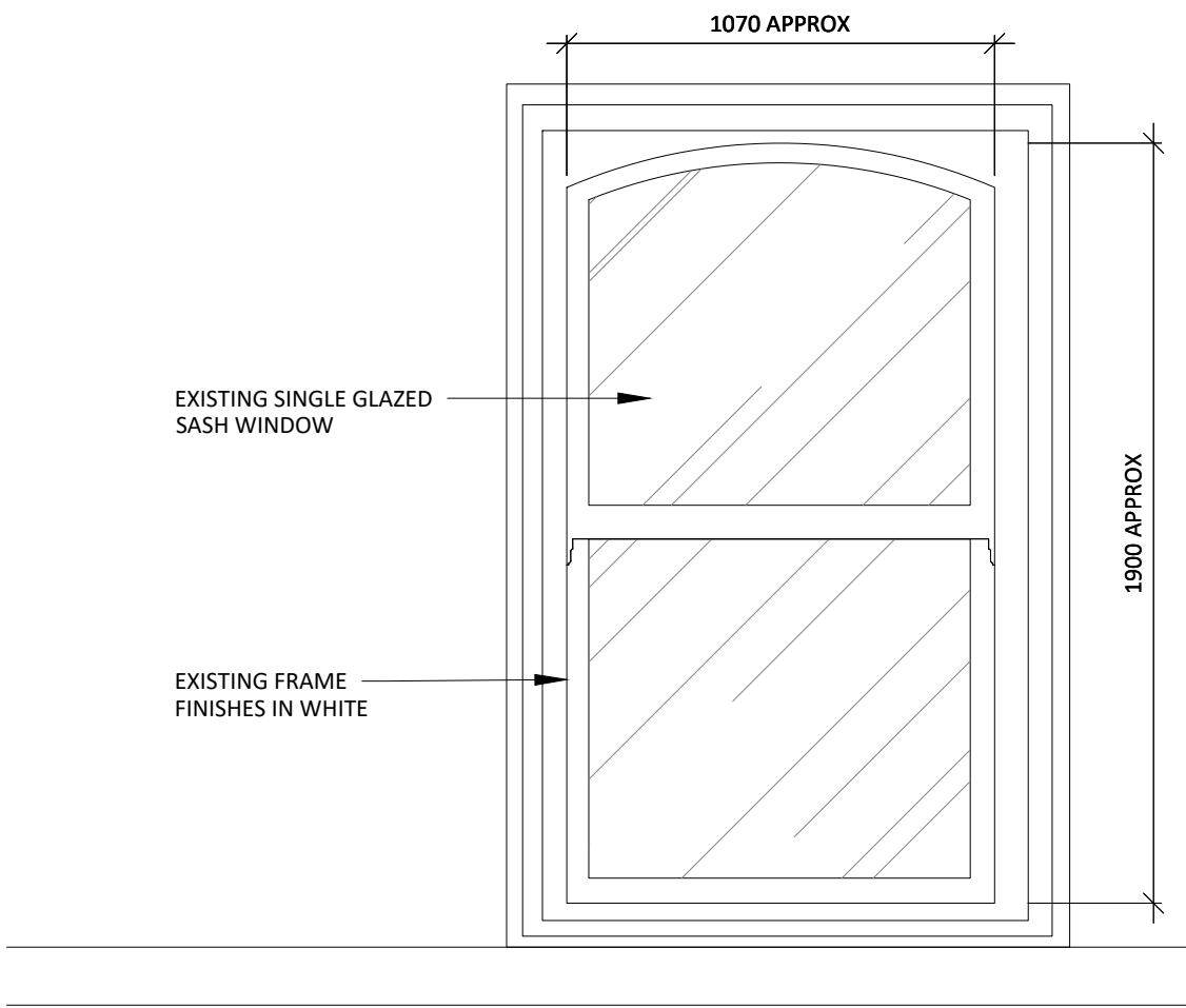
01 2nd FLOOR SASH WINDOW - TYPE B 511 SCALE 1:20 EXISTING ELEVATION
