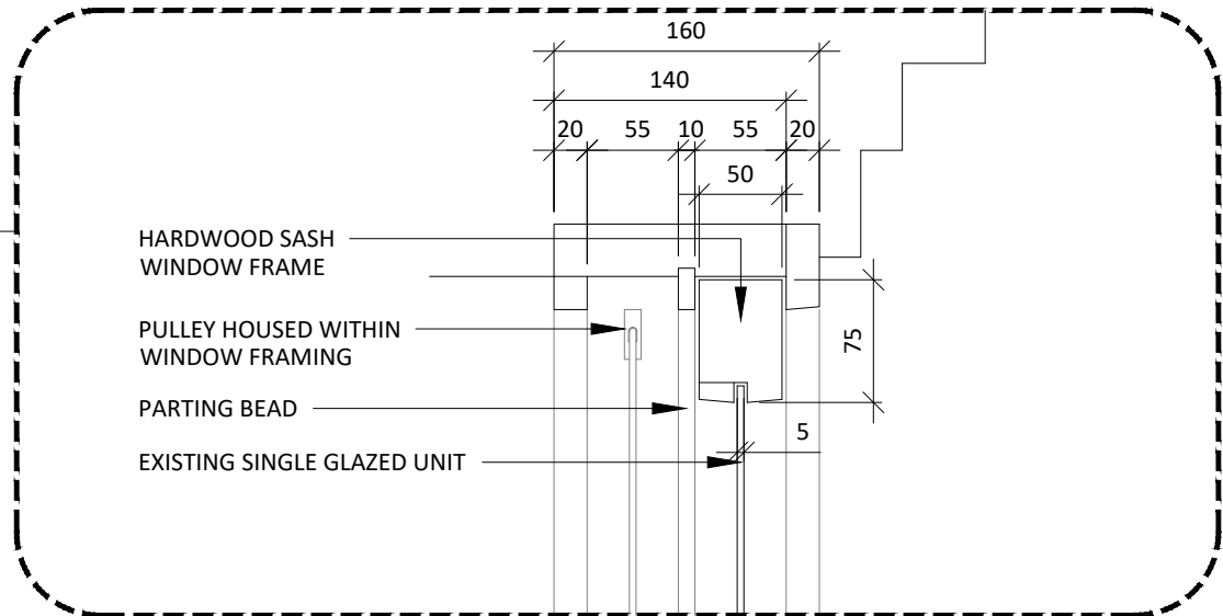
03a TYPE B WINDOW HEAD 511 SCALE 1:5 EXISTING SECTION
