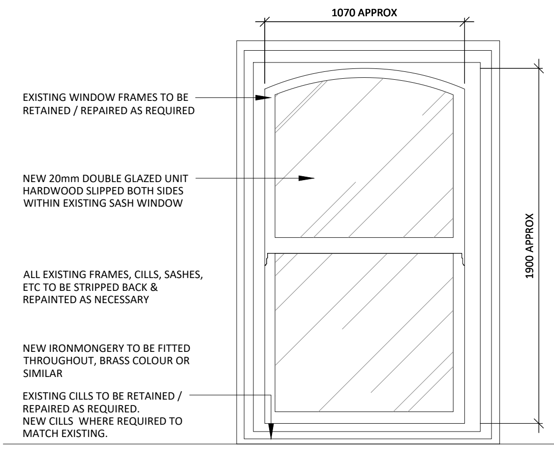
05 2nd FLOOR SASH WINDOW - TYPE B 511 SCALE 1:20 PROPOSED ELEVATION
