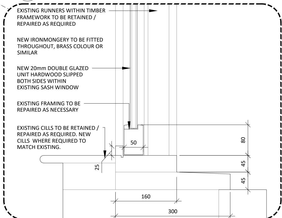
07c TYPE B WINDOW CILL 511 SCALE 1:5 PROPOSED SECTION
