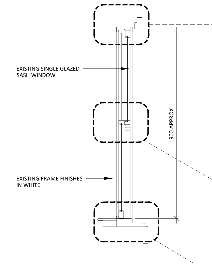
02 2nd FLOOR SASH WINDOW - TYPE B 511 SCALE 1:20 EXISTING SECTION
