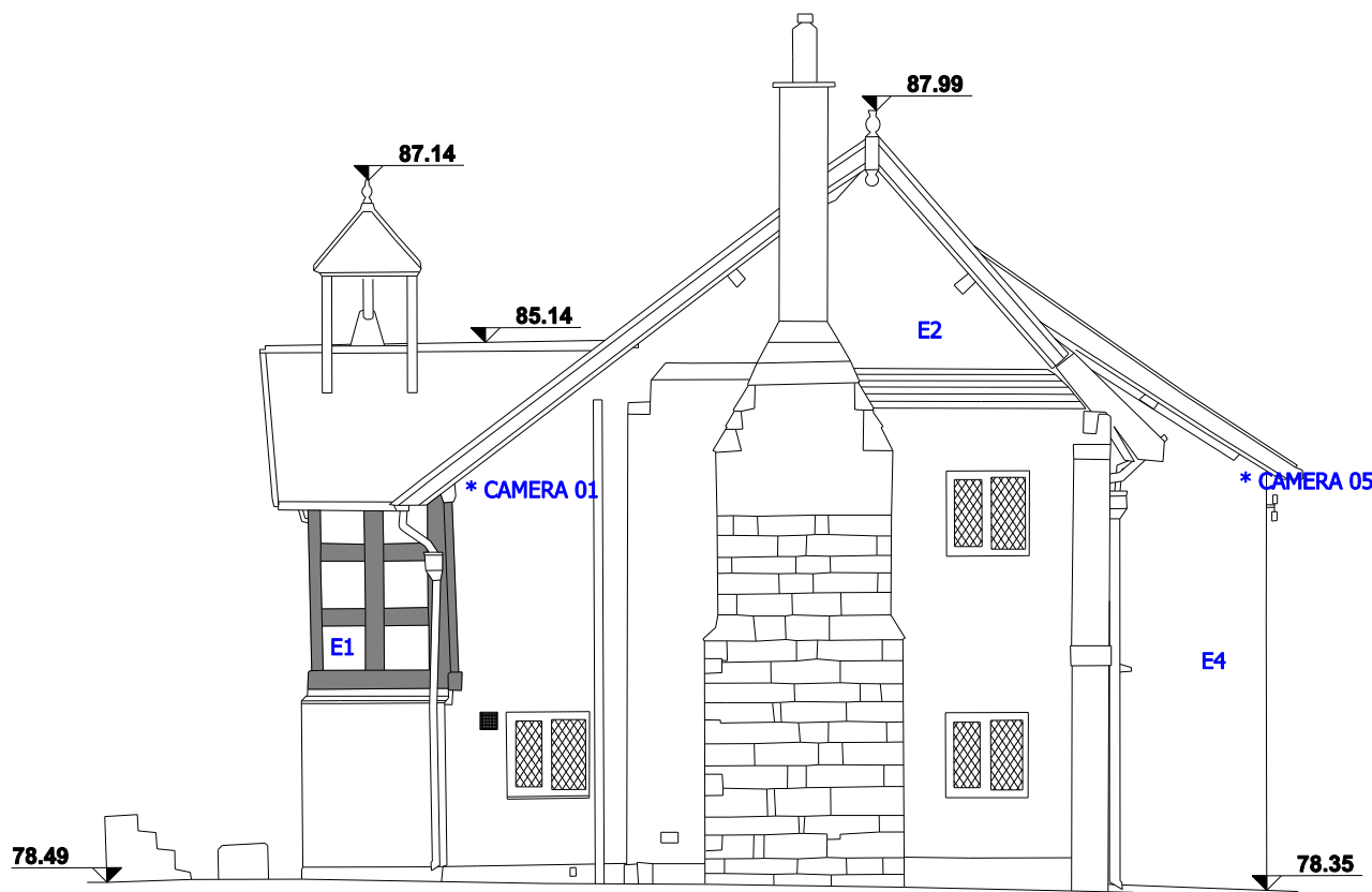
SOUTH ELEVATION AS PROPOSED
