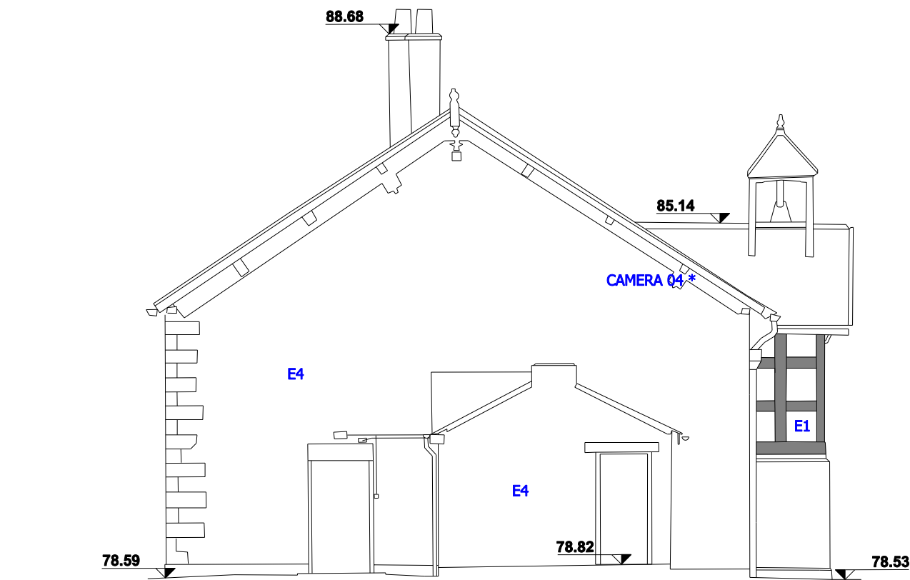
NORTH ELEVATION AS PROPOSED
