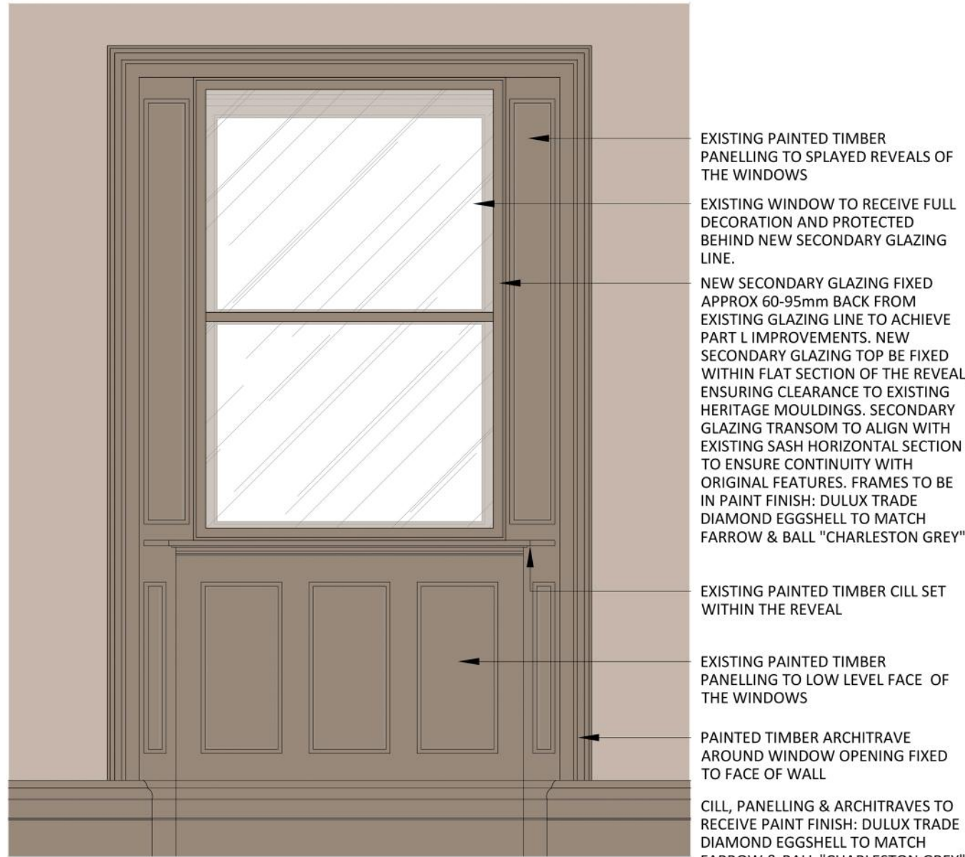
04 THIRD FLOOR PROPOSED WINDOW 573 SCALE - 1:20 @ A1 DETAIL ELEVATION
