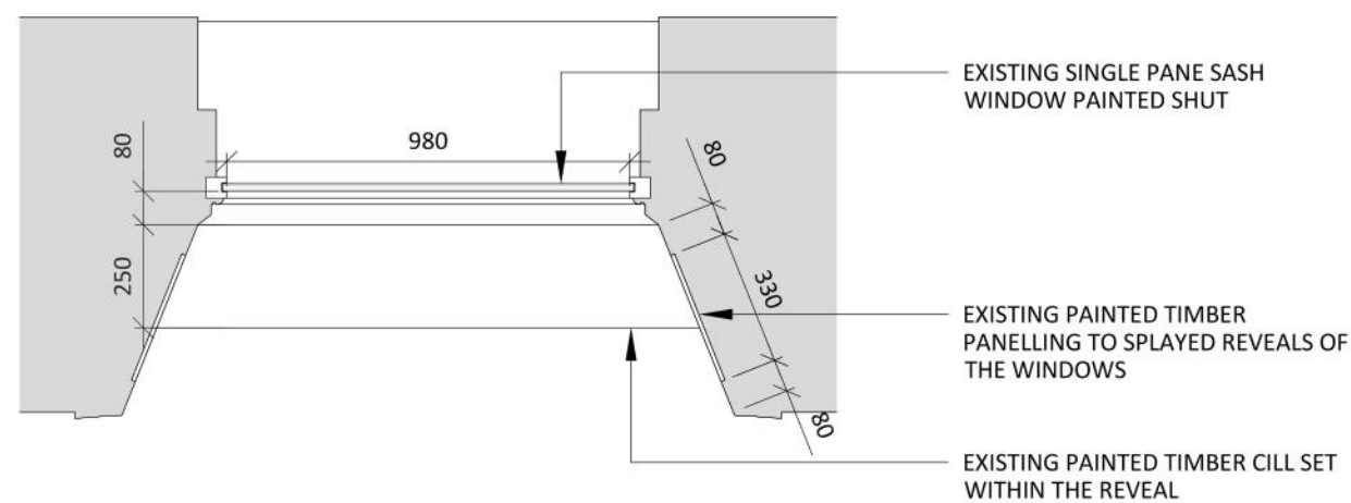
02 THIRD FLOOR EXISTING WINDOW PLAN 573 SCALE - 1:20 @ A1 DETAIL PLAN
