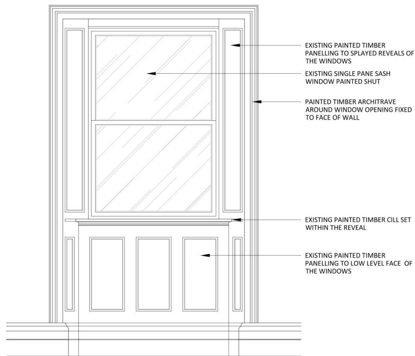
01 THIRD FLOOR EXISTING WINDOW ELEVATION 573 SCALE - 1:20 @ A1 DETAIL ELEVATION
