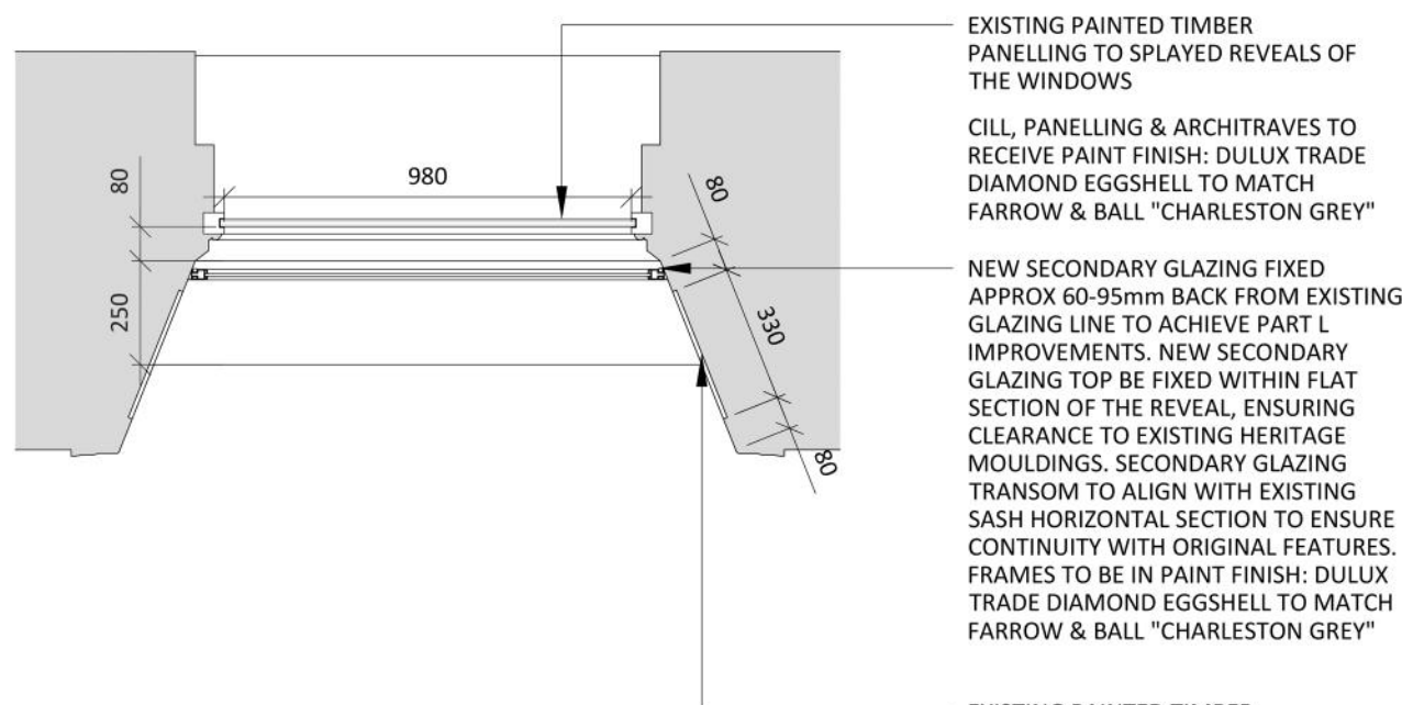
05 THIRD FLOOR PROPOSED WINDOW 573 SCALE - 1:20 @ A1 DETAIL PLAN
