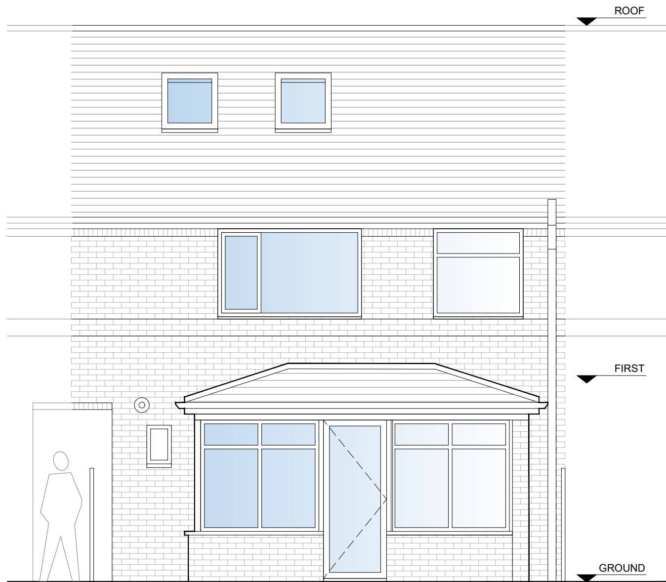
• Existing elevation 1
