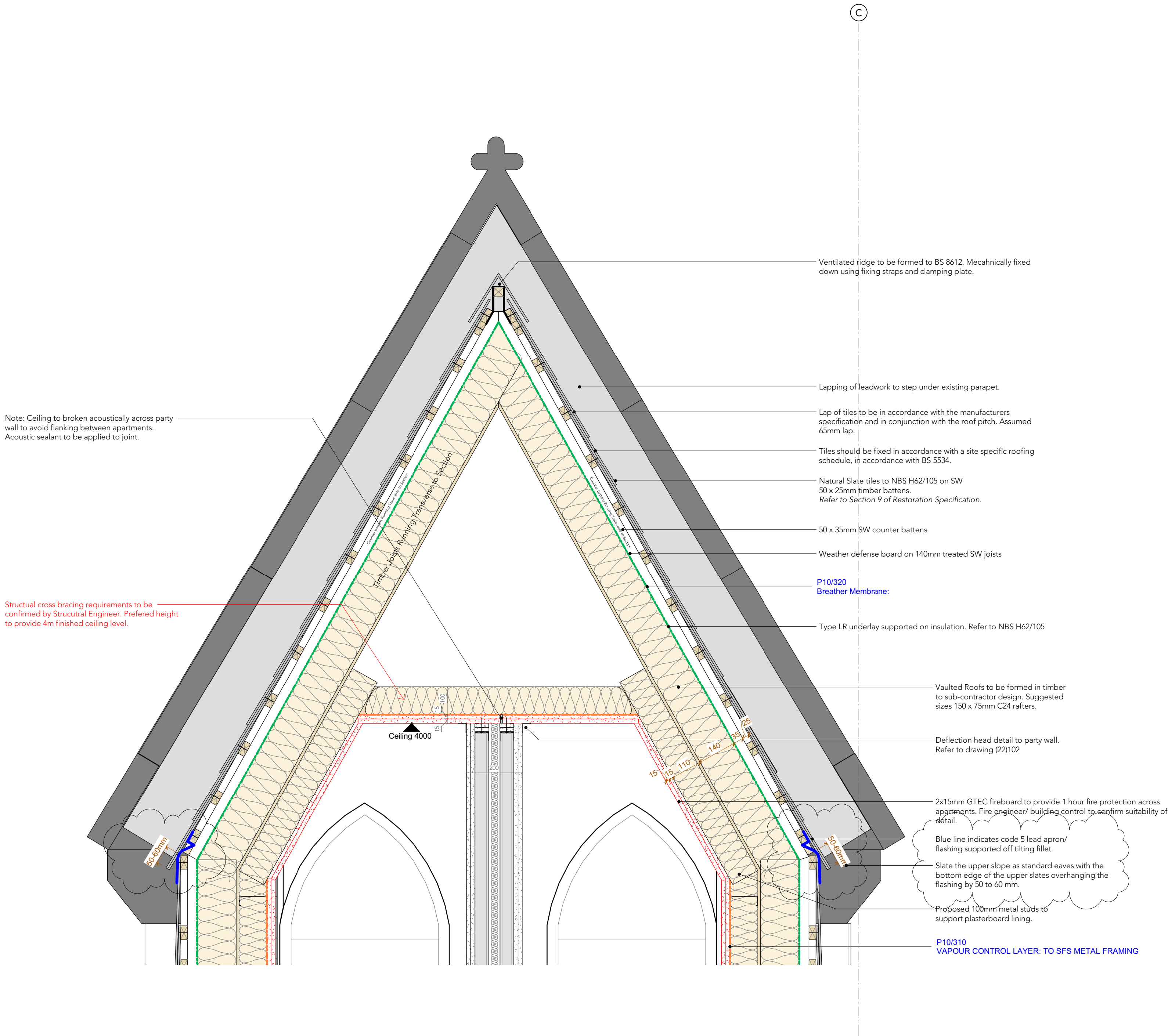
Section J - Typical Dormer Roof & Party Wall Detail
