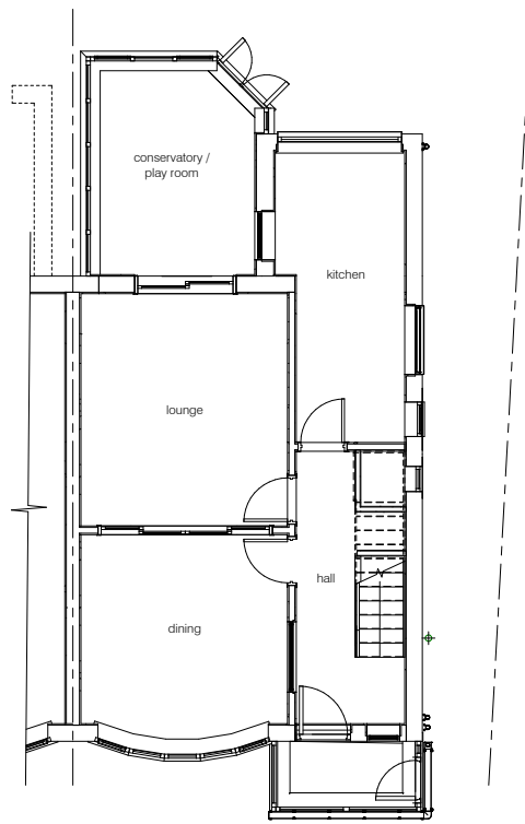
00 existing ground floor 1 : 50
