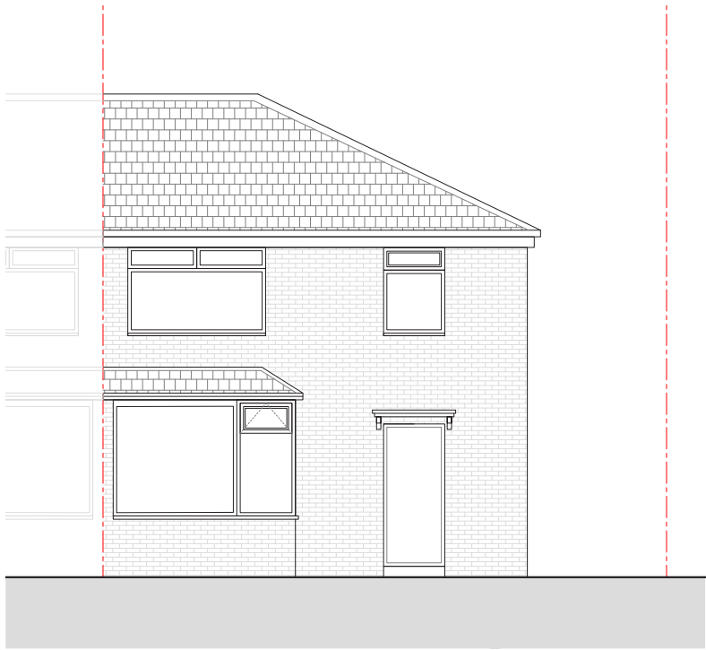
EXISTING FRONT ELEVATION 1:100 @ A3
