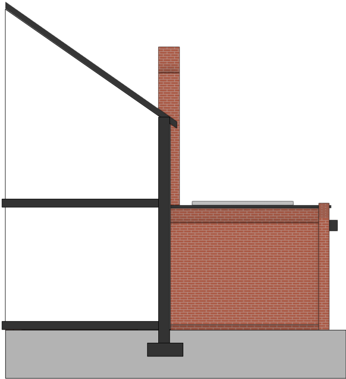
PROPOSED SIDE ELEVATION FROM ATTACHED PROPERTY
