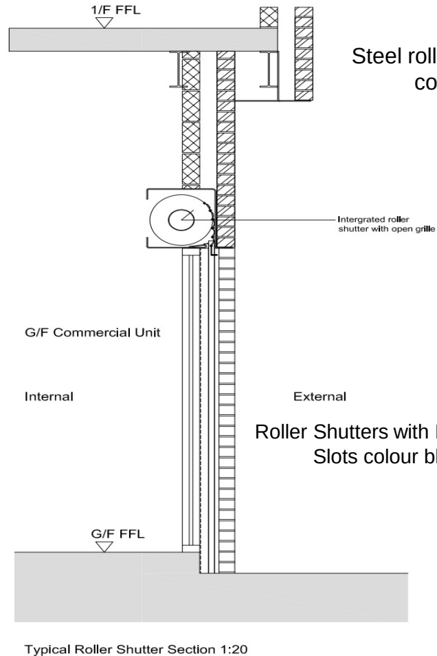
Typical Roller Shutter Section 1:20
