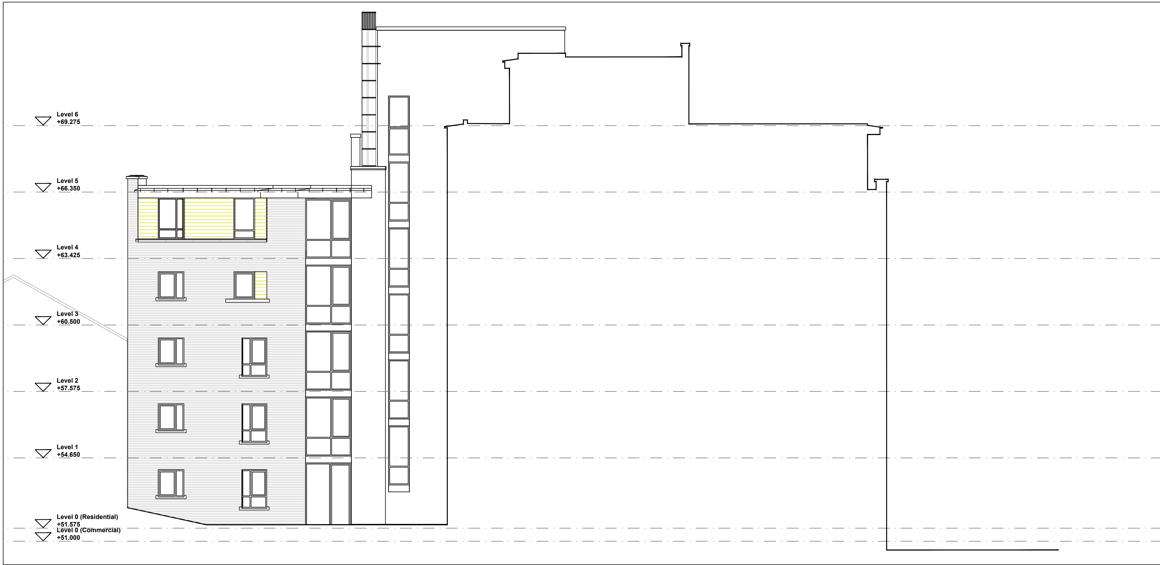
[5] Sectional Elevation A 1:100
