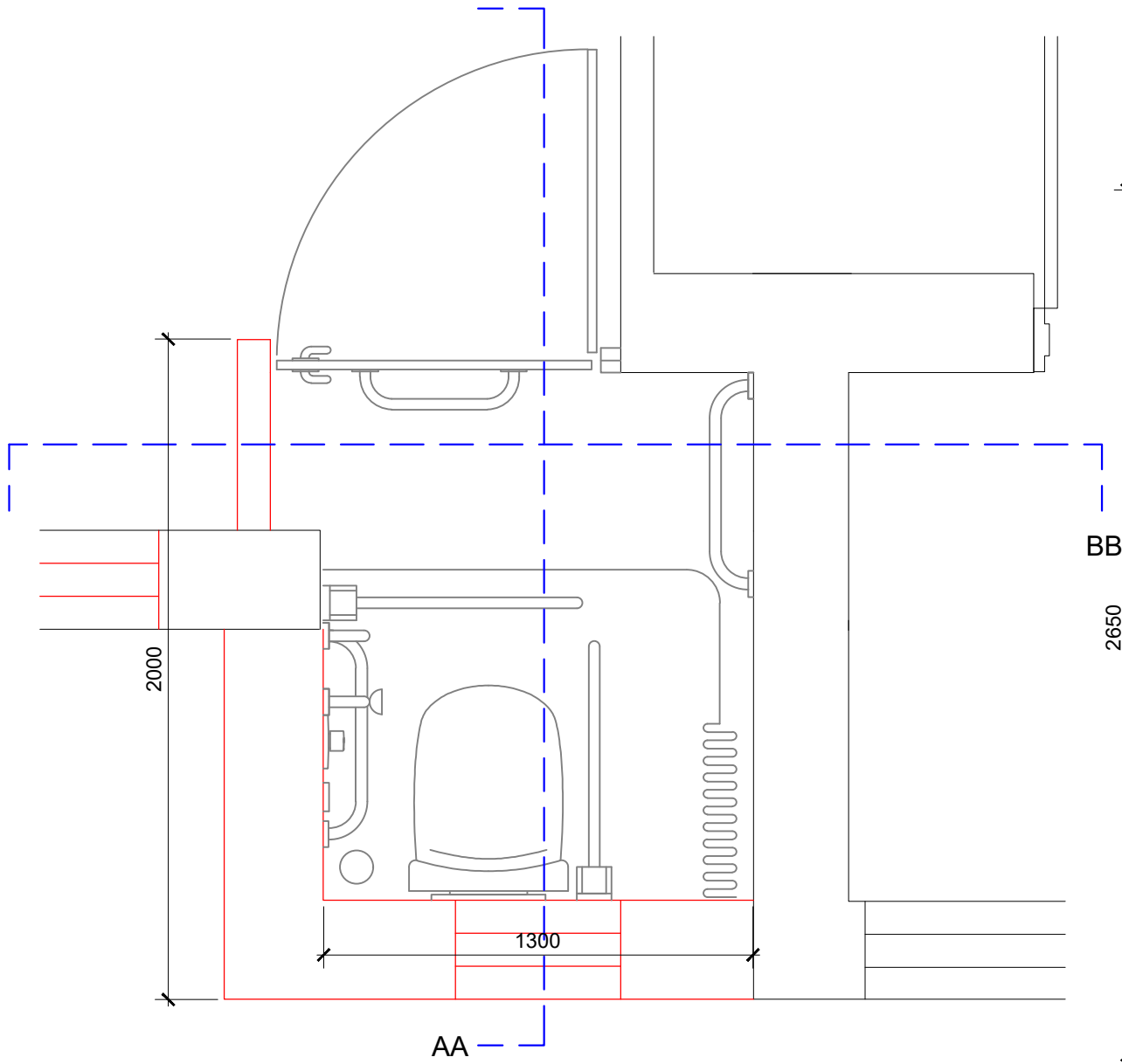
Wet Room as Proposed 1:20
