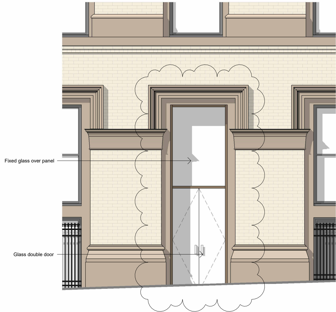
1 Bloom Street Phase 3 Entrance Detail 1 : 50
