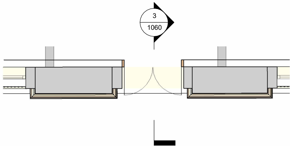
2 Bloom Street Phase 3 Entrance Plan 1 : 50
