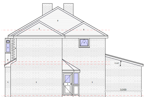
PROPOSED GA SIDE ELEVATION 1 @1:100
