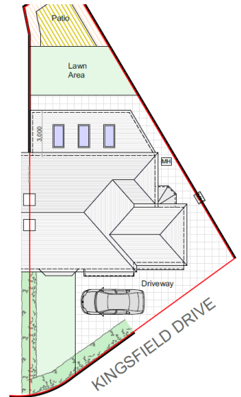
PROPOSED GA SITE PLAN @1:200
