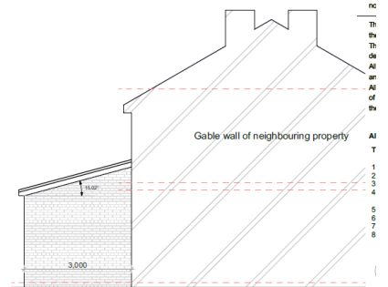
PROPOSED GA SIDE ELEVATION 2 @1:100
