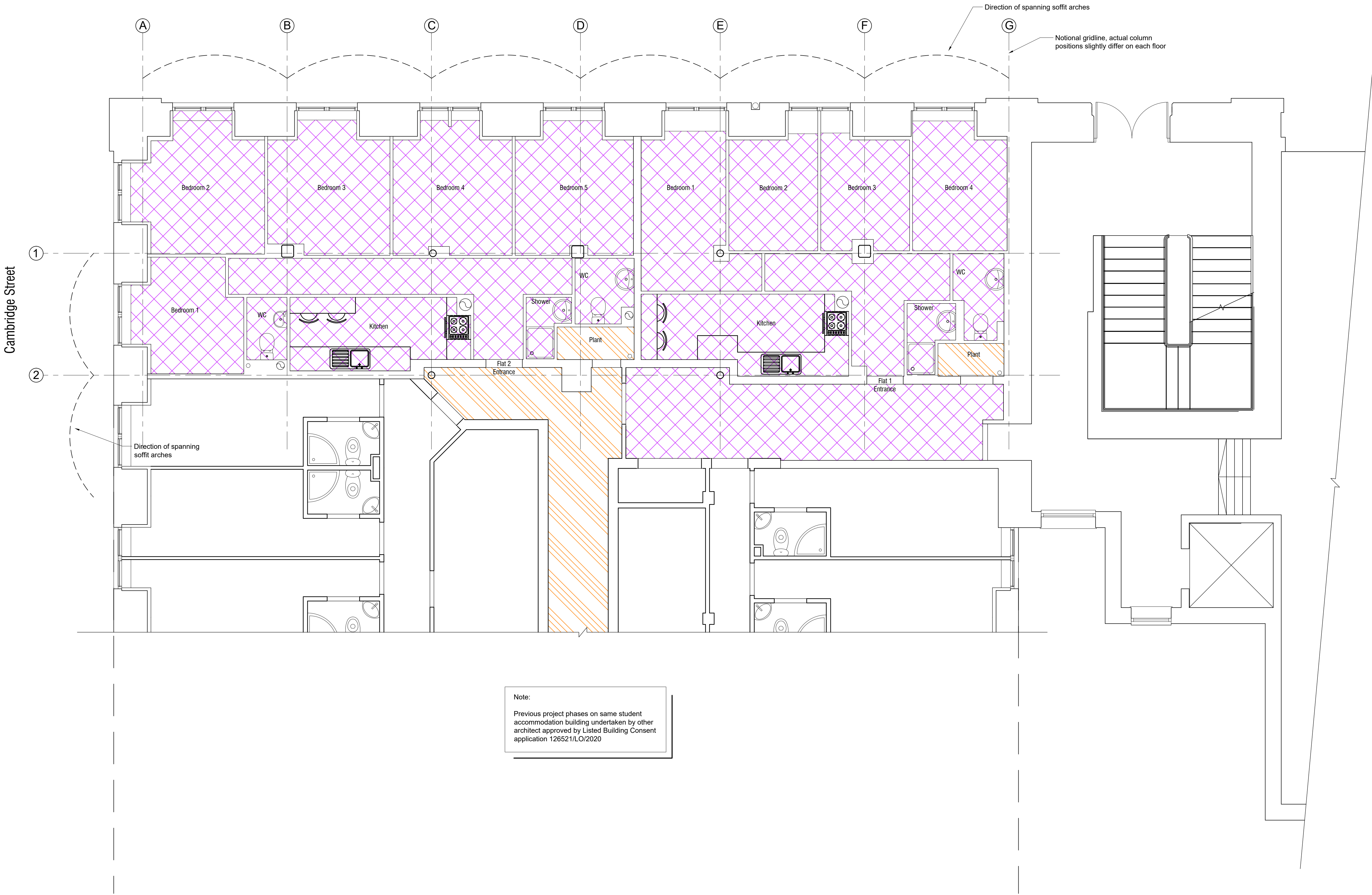
Existing Ground Floor Ceiling [Level 0] Typical Ceiling Plan Scale 1:50
