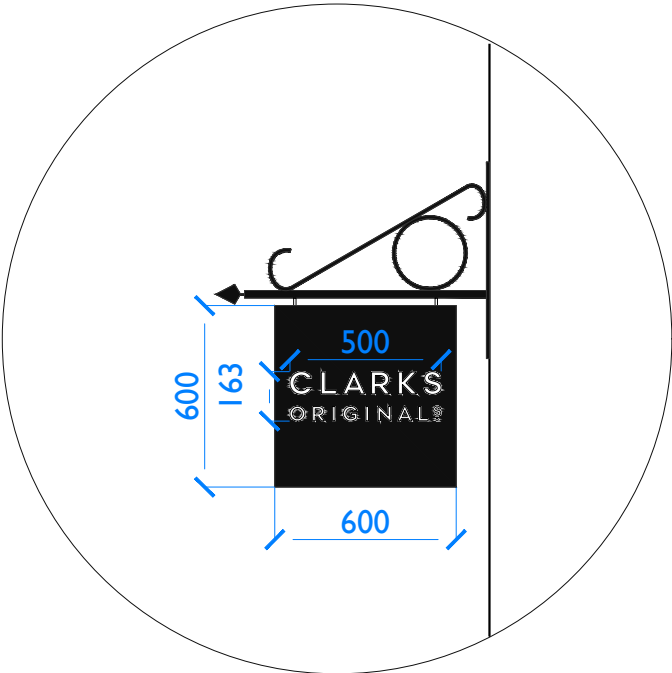
PROPOSED PROJECTING SIGN SIDE ELEVATION (1:25 @ A3)
