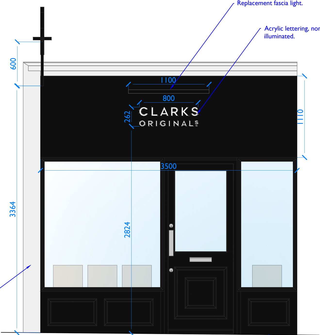
PROPOSED SHOP FRONT ELEVATION (1:25 @ A3)
