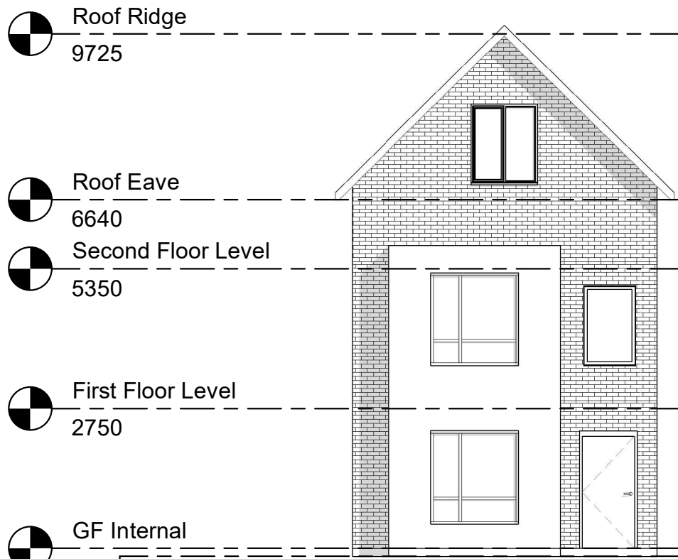
1 Front Existing 1 : 100
