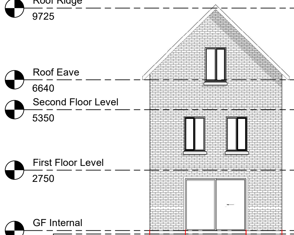
3 Rear Existing 1 : 100
