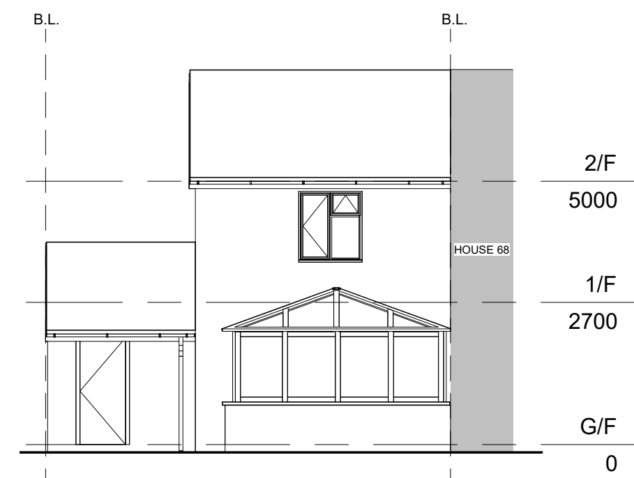
2 Existing Rear Elevation 1 : 100
