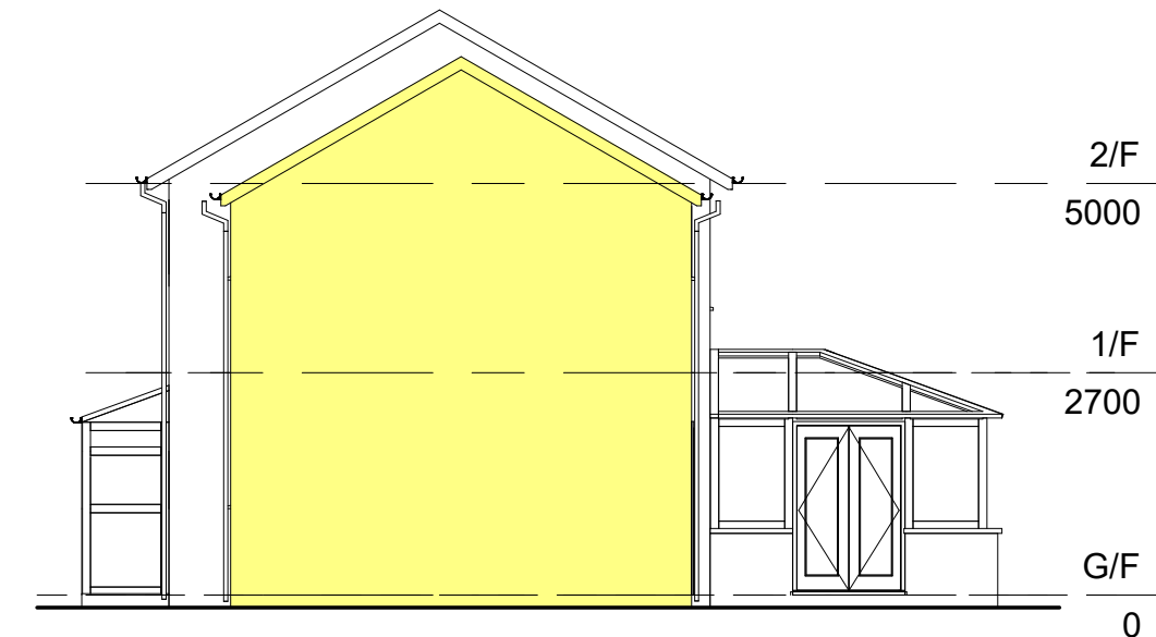
10 Proposed Side Elevation 1 : 100
