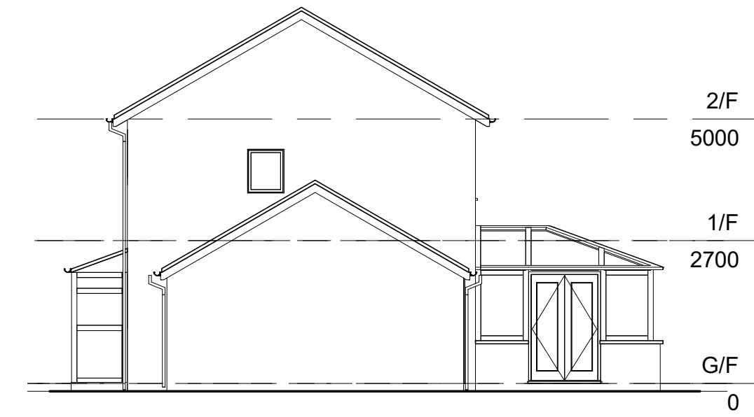
3 Existing Side Elevation 1 1 : 100
