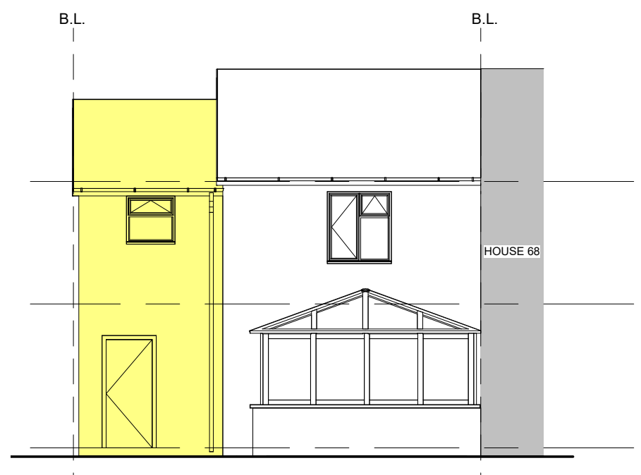
9 Proposed Rear Elevation 1 : 100
