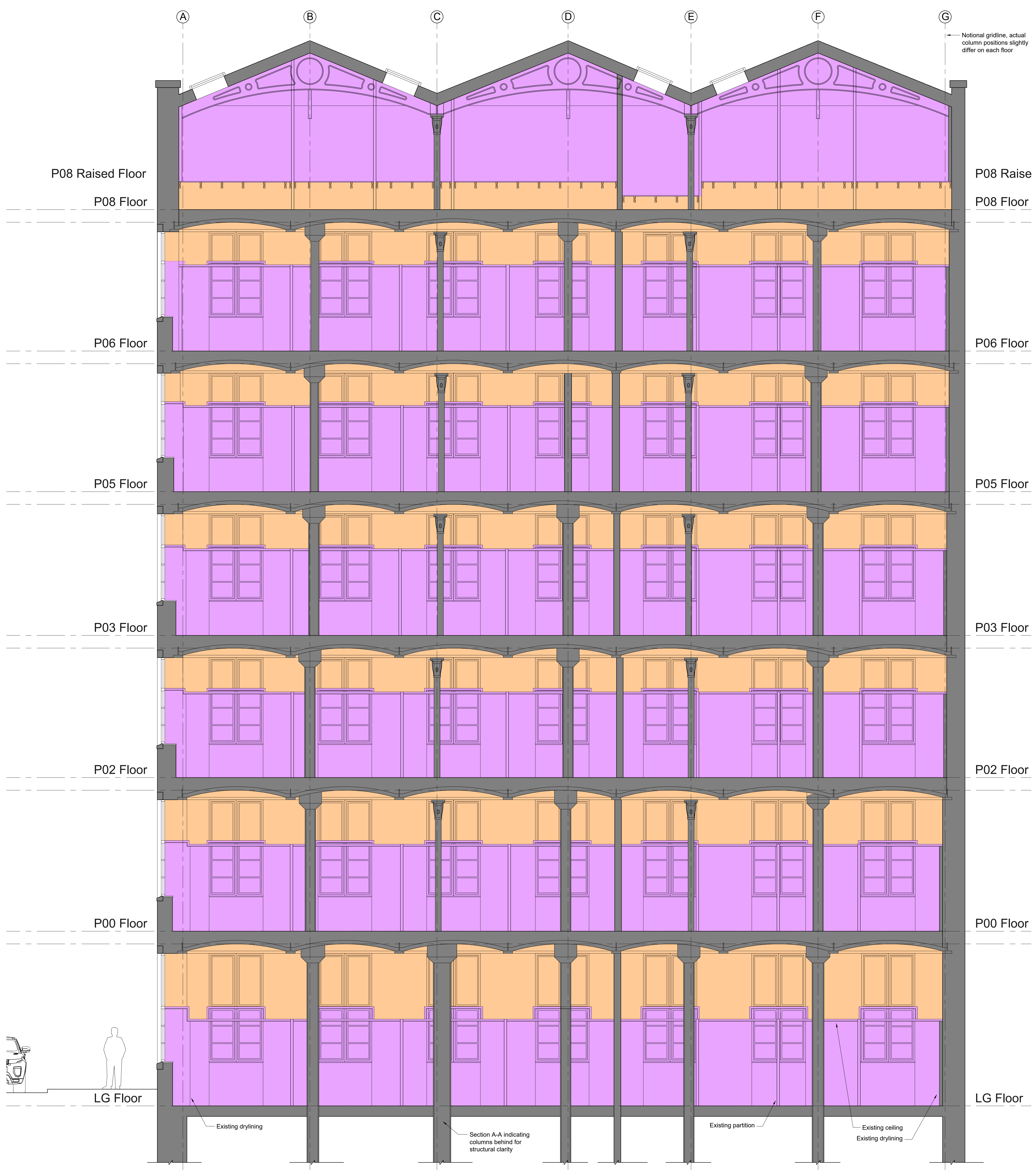
Existing Section A-A Scale 1:50
