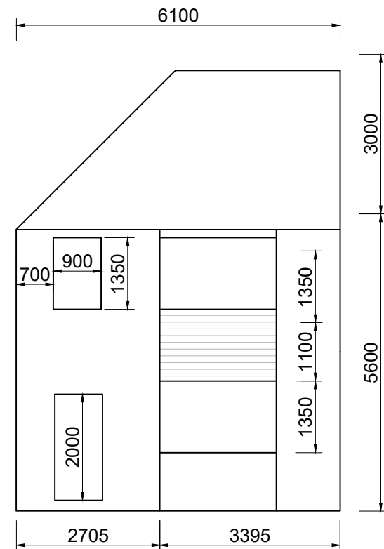
Front Elevation as Existing
