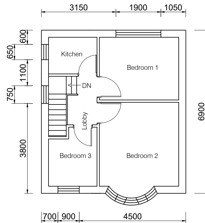
First Floor Plan as Existing
