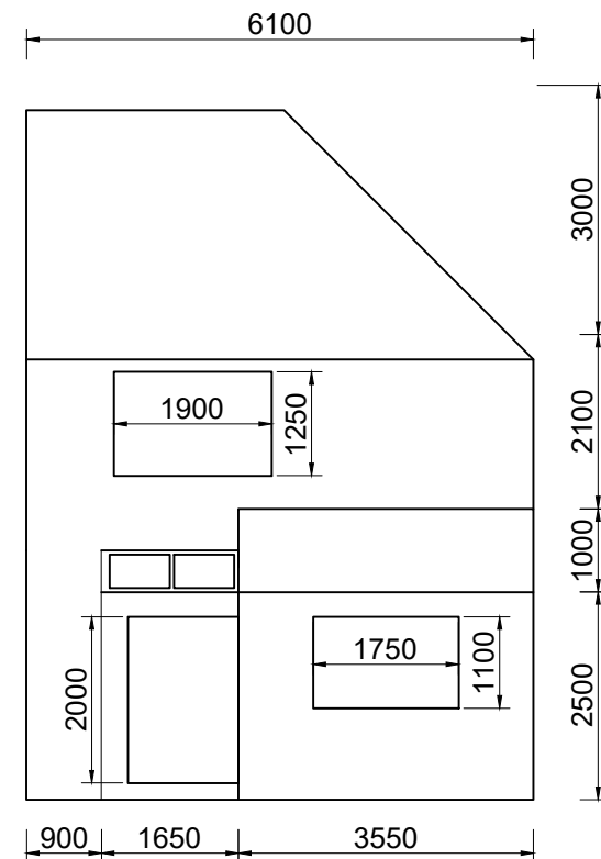
Rear Elevation as Existing
