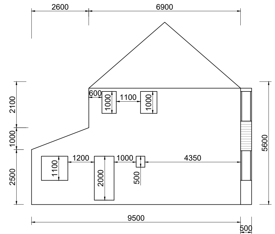
South Elevation as Existing
