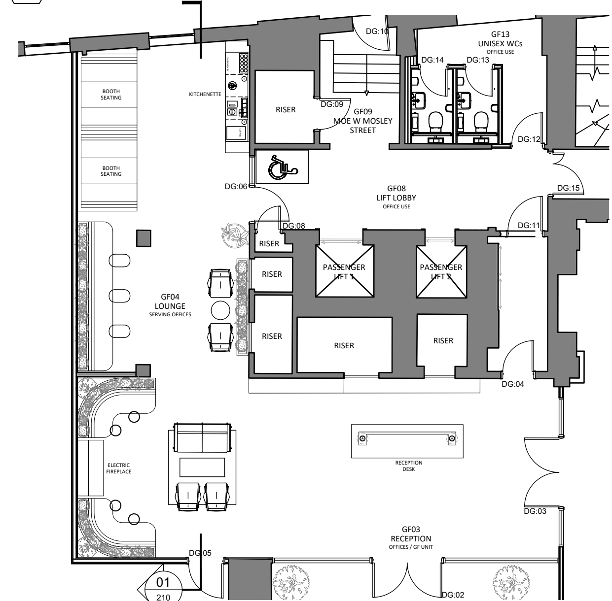
02 GROUND FLOOR LOUNGE SECTION SCALE - 1:100 @ A1
