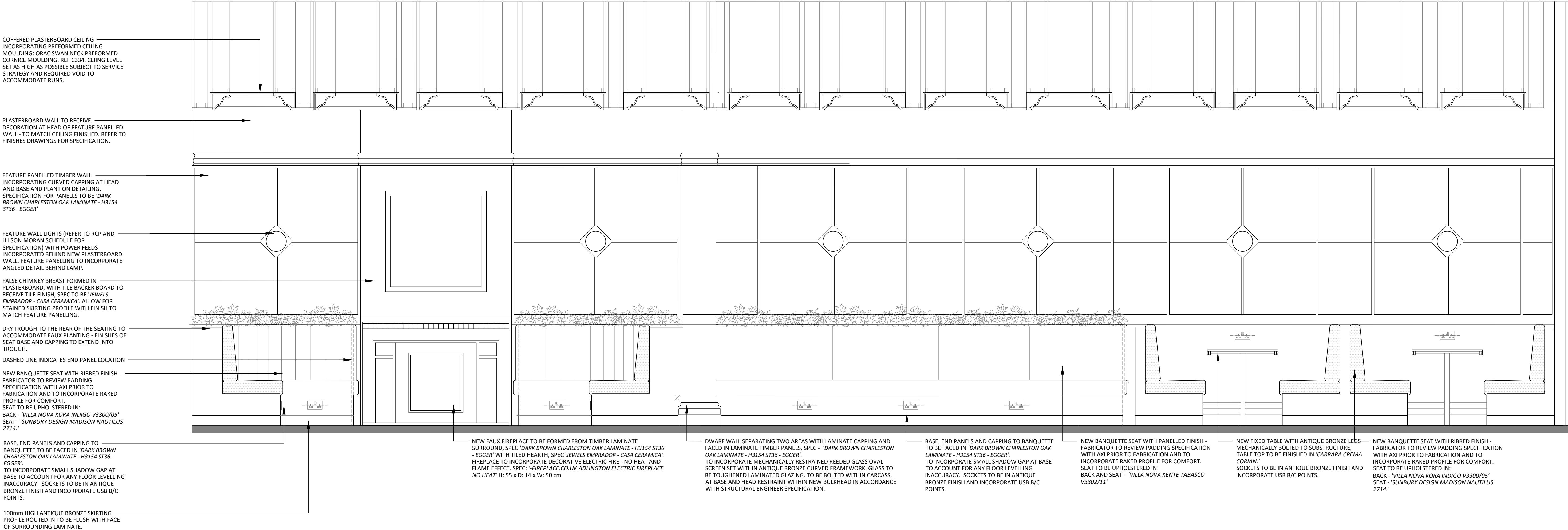
01 GROUND FLOOR LOUNGE SECTION DETAIL SCALE - 1:20 @ A1
