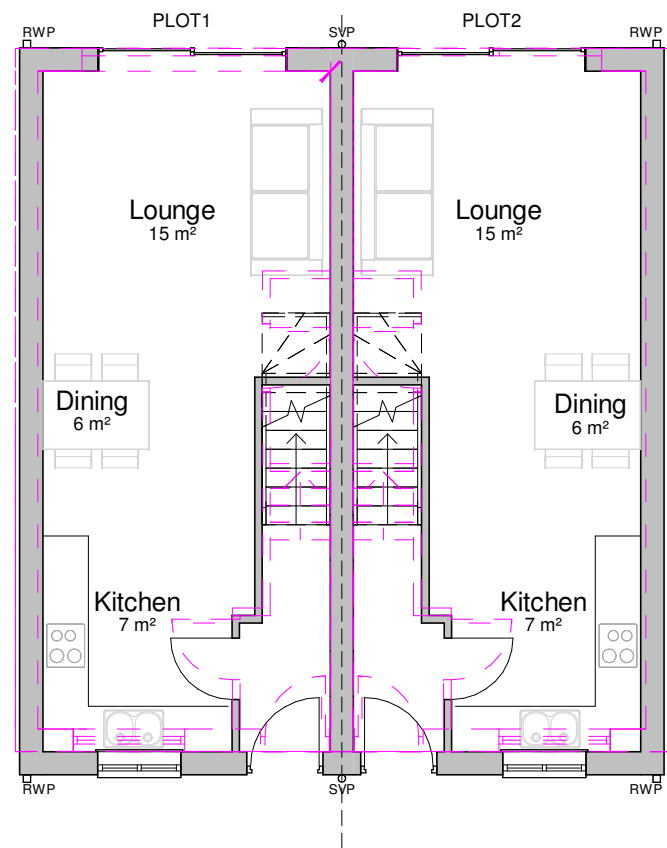
1 As-built Ground Floor Plan 1 : 100
