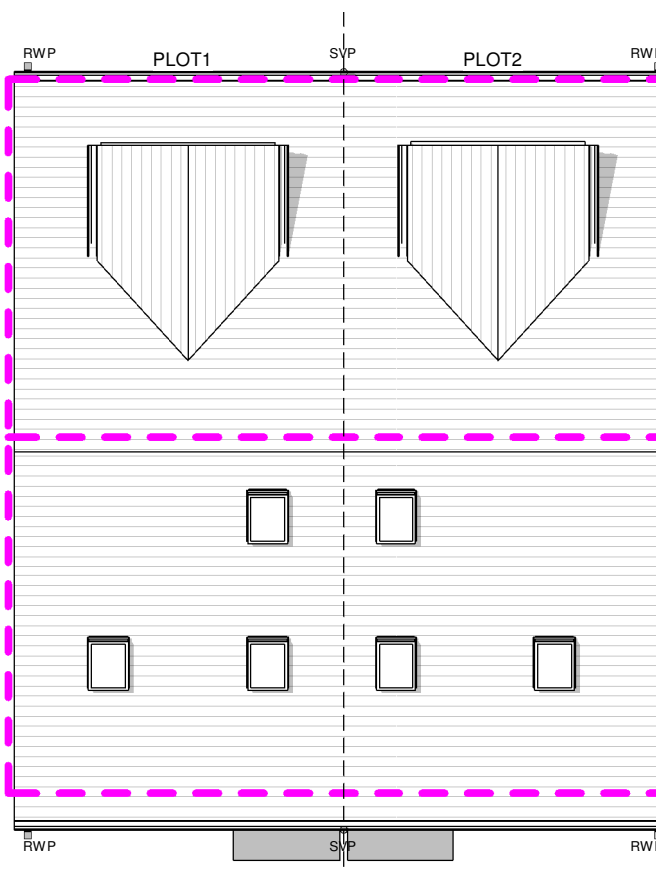
4 As-built Roof Plan 1 : 100
