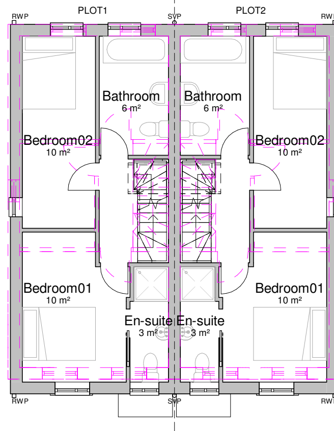
2 As-built First Floor Plan 1 : 100
