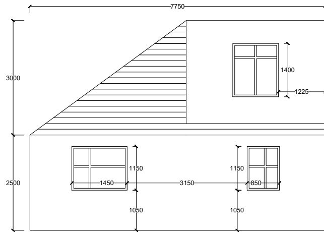
Rear Elevation as Existing
