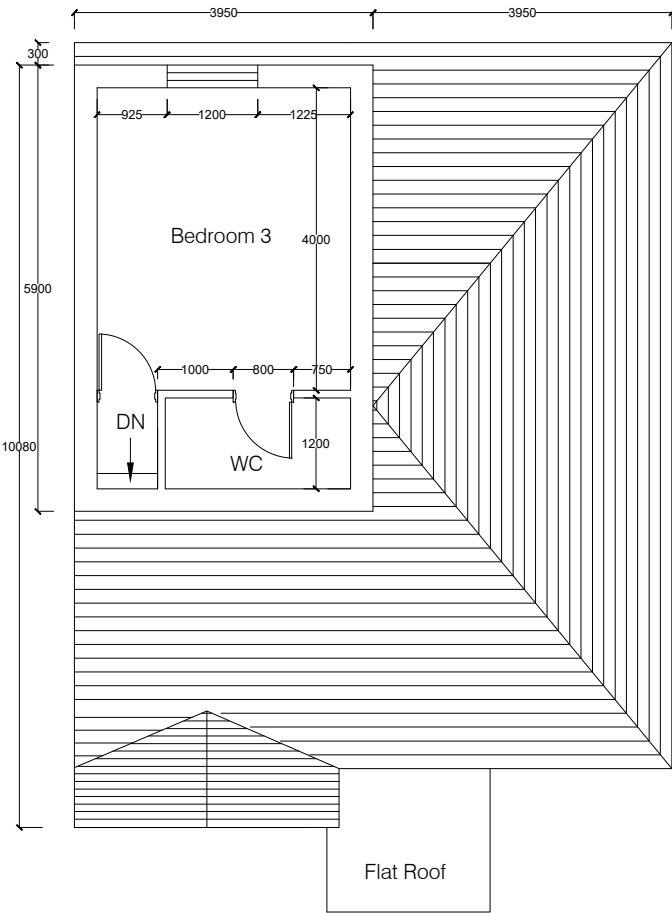
Dormer Plan as Existing
