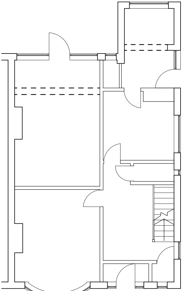
GROUND FLOOR SCALE 1:100 UID - E003
