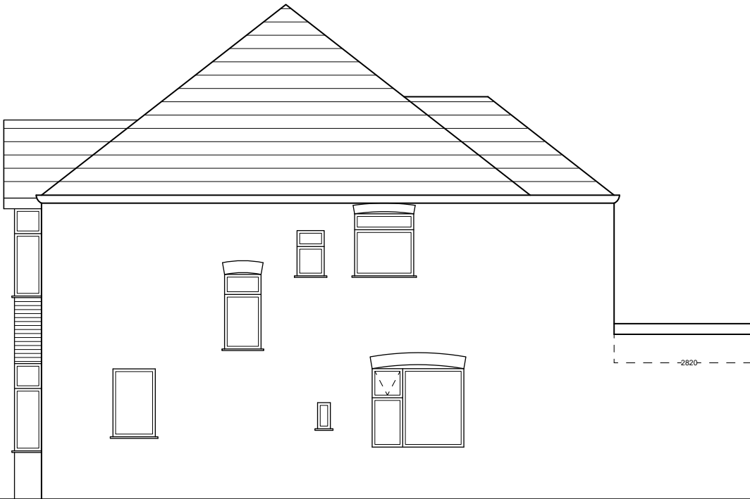
SOUTH ELEVATION SCALE 1:100 UID - P008
