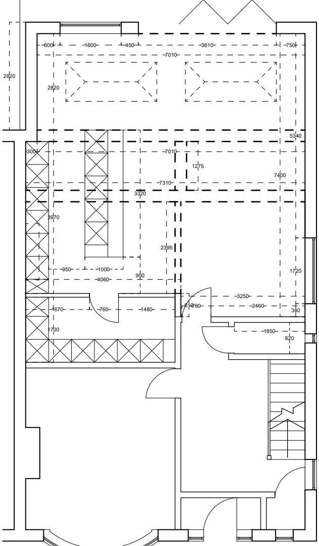
GROUND FLOOR SCALE 1:100 UID - P003
