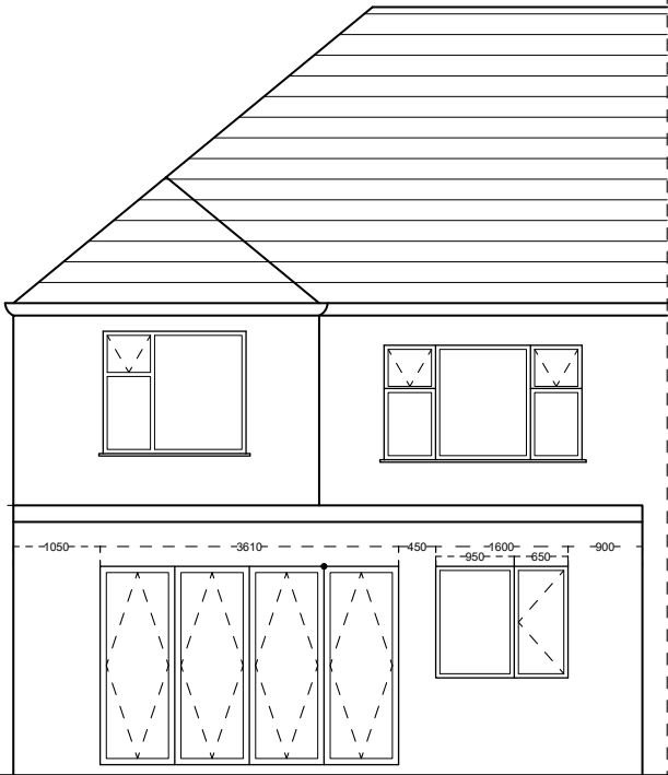
EAST ELEVATION SCALE 1:100 UID - P007
