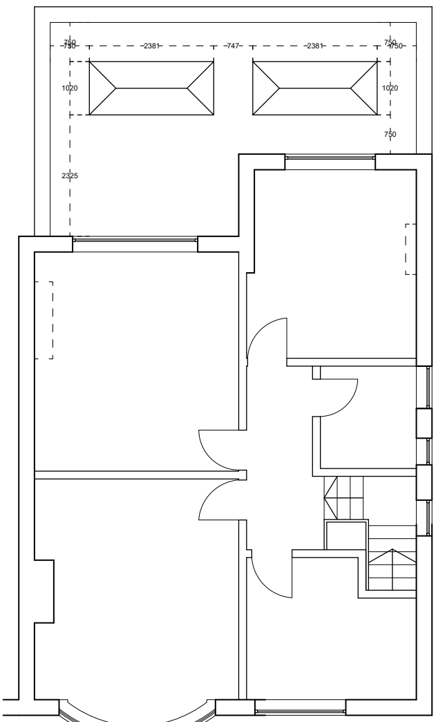
FIRST FLOOR SCALE 1:100 UID - P004
