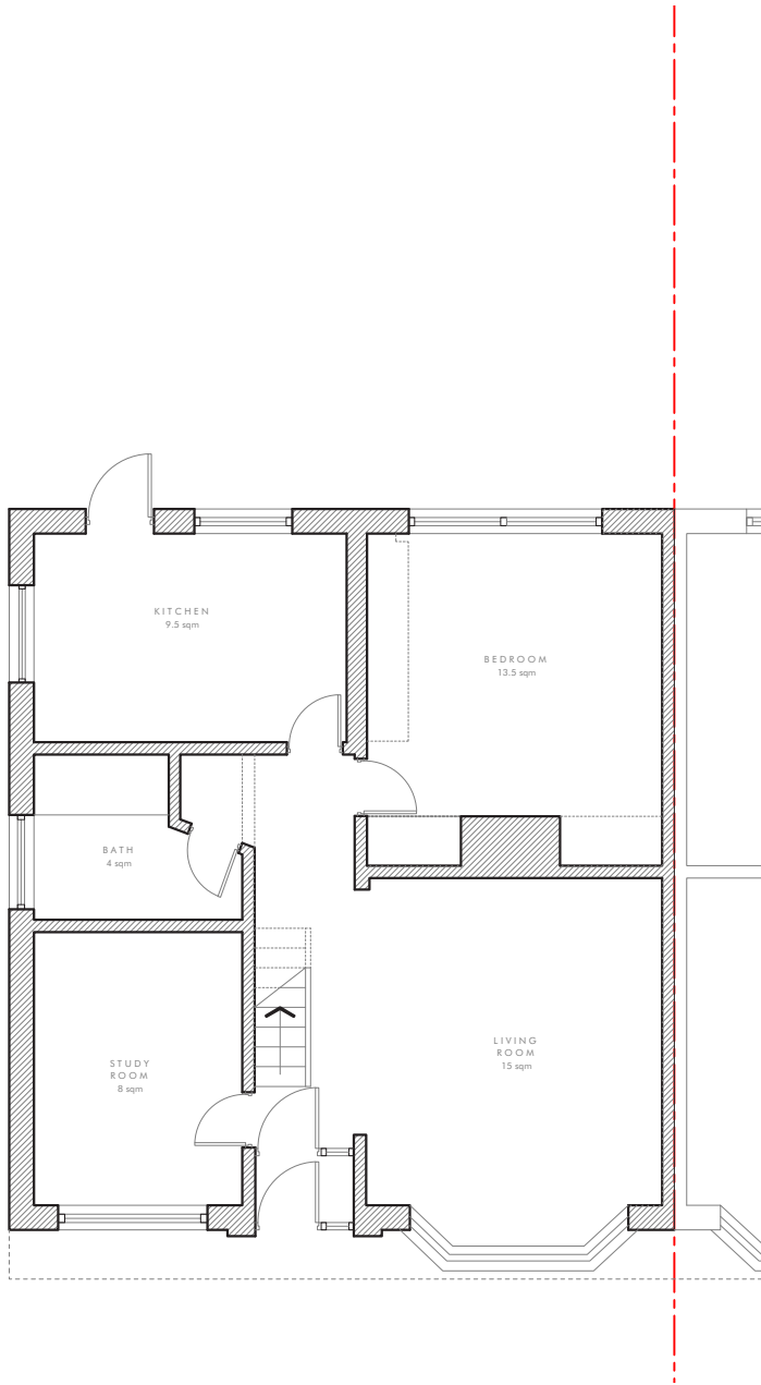
EXISTING GROUND FLOOR PLAN 1:100 @ A3
